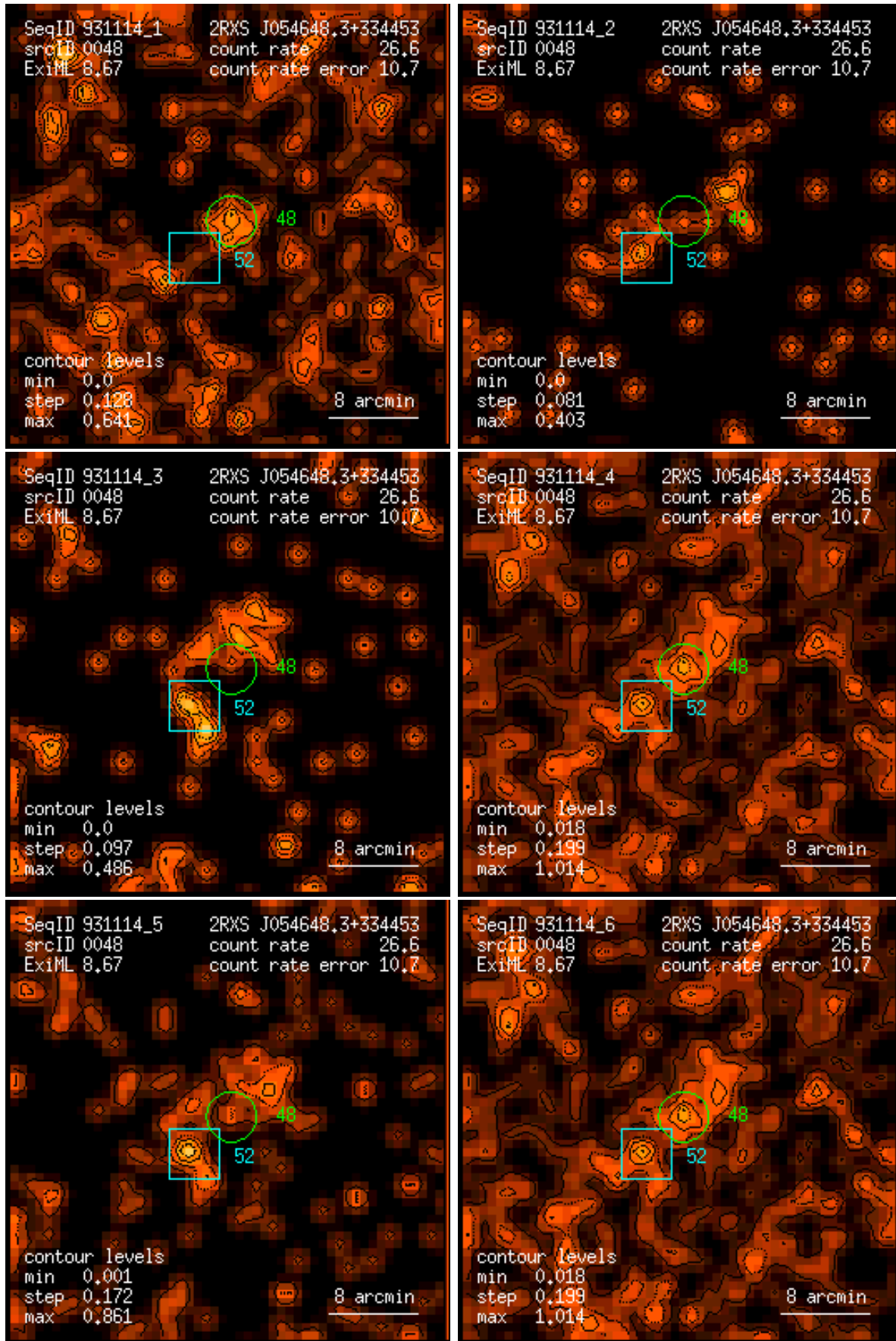
Figure 48: RASS 931114: detection 0048: band rate images, Gaussian filter: (1) PSPC channels 11 – 41, (2) 52 – 90, (3) 91 – 201, (4) 11 – 235, (5) 52 – 201, (6) 11 – 201. Broad band rates in counts/ks. Band rate contour levels in counts/ks/arcmin 2 .
