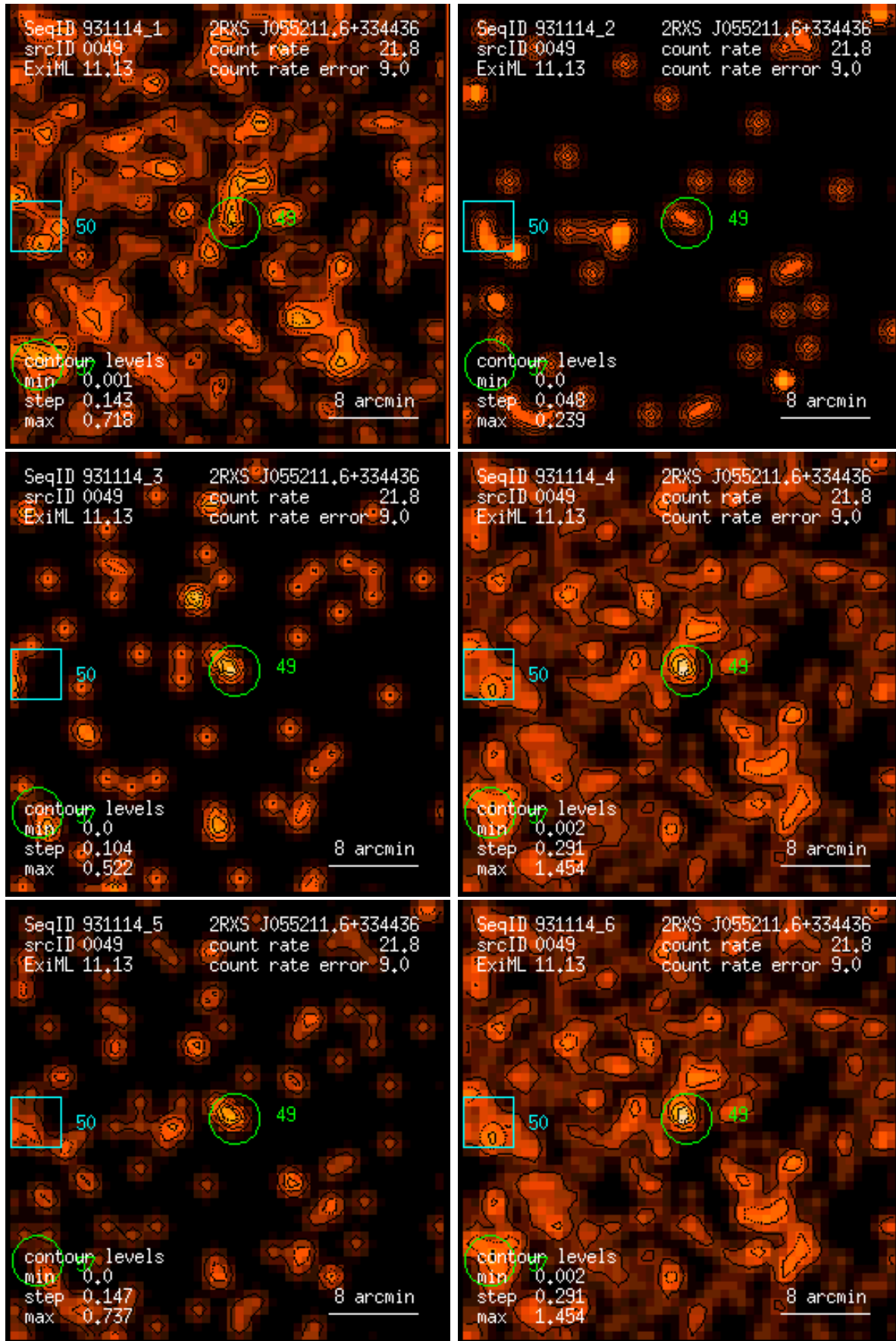
Figure 49: RASS 931114: detection 0049: band rate images, Gaussian filter: (1) PSPC channels 11 – 41, (2) 52 – 90, (3) 91 – 201, (4) 11 – 235, (5) 52 – 201, (6) 11 – 201. Broad band rates in counts/ks. Band rate contour levels in counts/ks/arcmin 2 .
