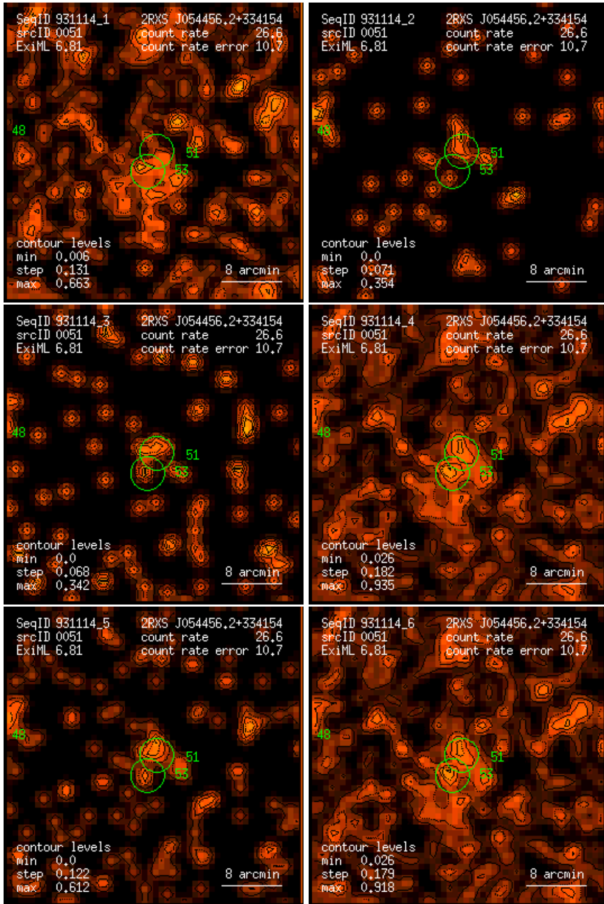
Figure 51: RASS 931114: detection 0051: band rate images, Gaussian filter: (1) PSPC channels 11 – 41, (2) 52 – 90, (3) 91 – 201, (4) 11 – 235, (5) 52 – 201, (6) 11 – 201. Broad band rates in counts/ks. Band rate contour levels in counts/ks/arcmin 2 .
