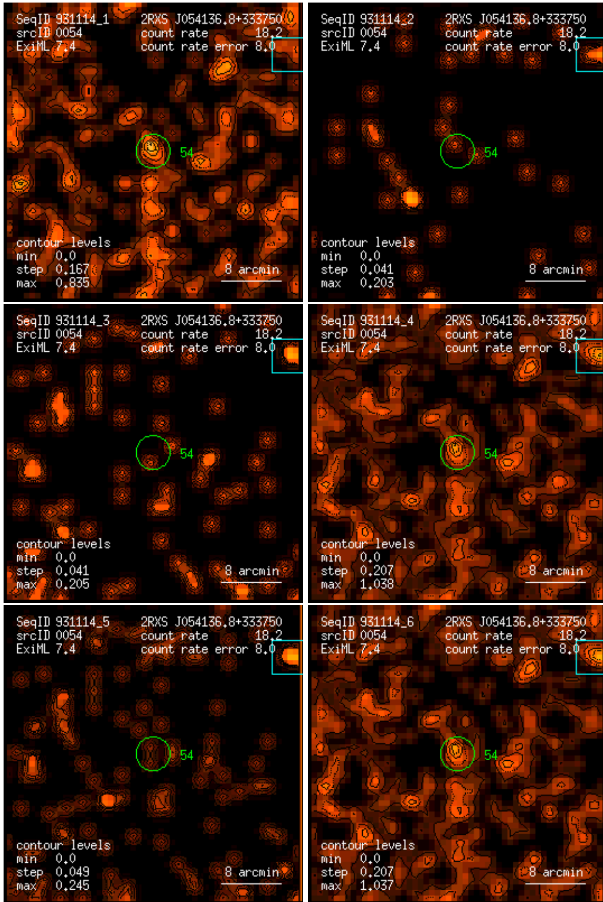
Figure 54: RASS 931114: detection 0054: band rate images, Gaussian filter: (1) PSPC channels 11 – 41, (2) 52 – 90, (3) 91 – 201, (4) 11 – 235, (5) 52 – 201, (6) 11 – 201. Broad band rates in counts/ks. Band rate contour levels in counts/ks/arcmin 2 .
