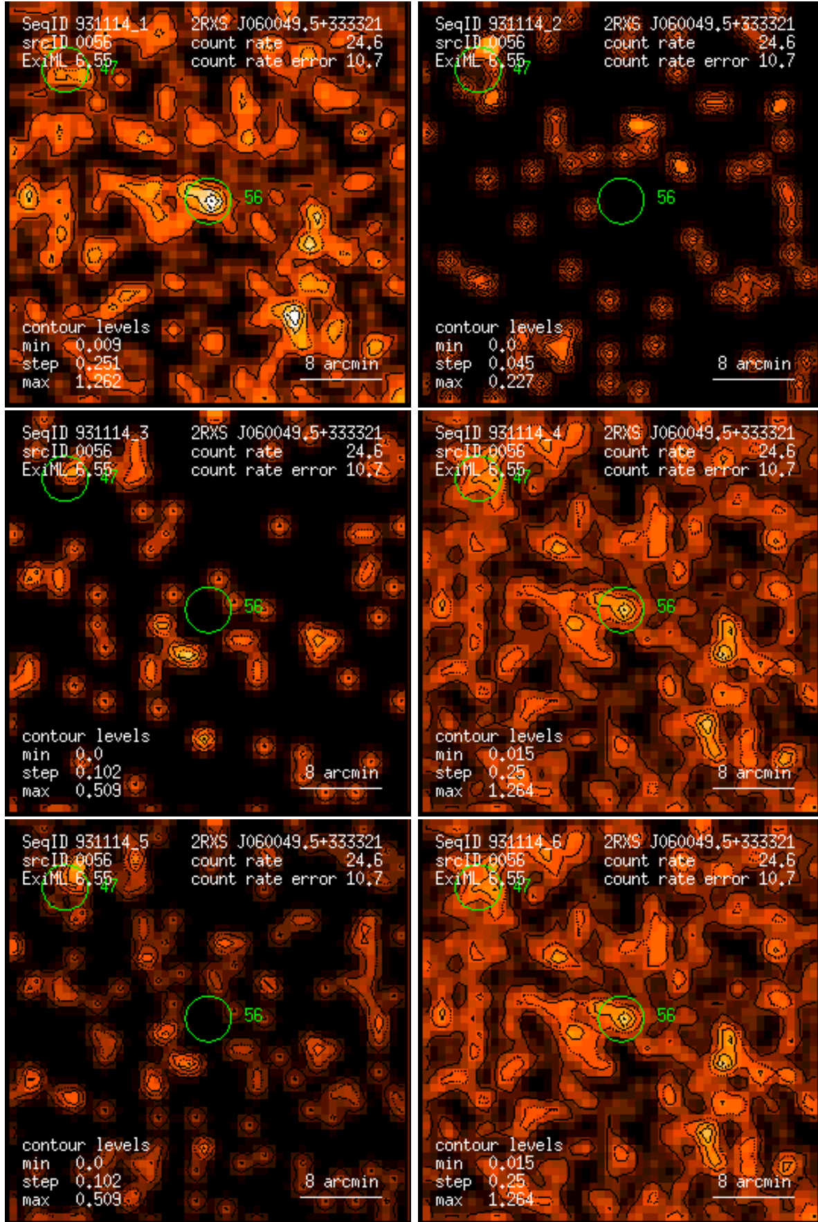
Figure 56: RASS 931114: detection 0056: band rate images, Gaussian filter: (1) PSPC channels 11 – 41, (2) 52 – 90, (3) 91 – 201, (4) 11 – 235, (5) 52 – 201, (6) 11 – 201. Broad band rates in counts/ks. Band rate contour levels in counts/ks/arcmin 2 .
