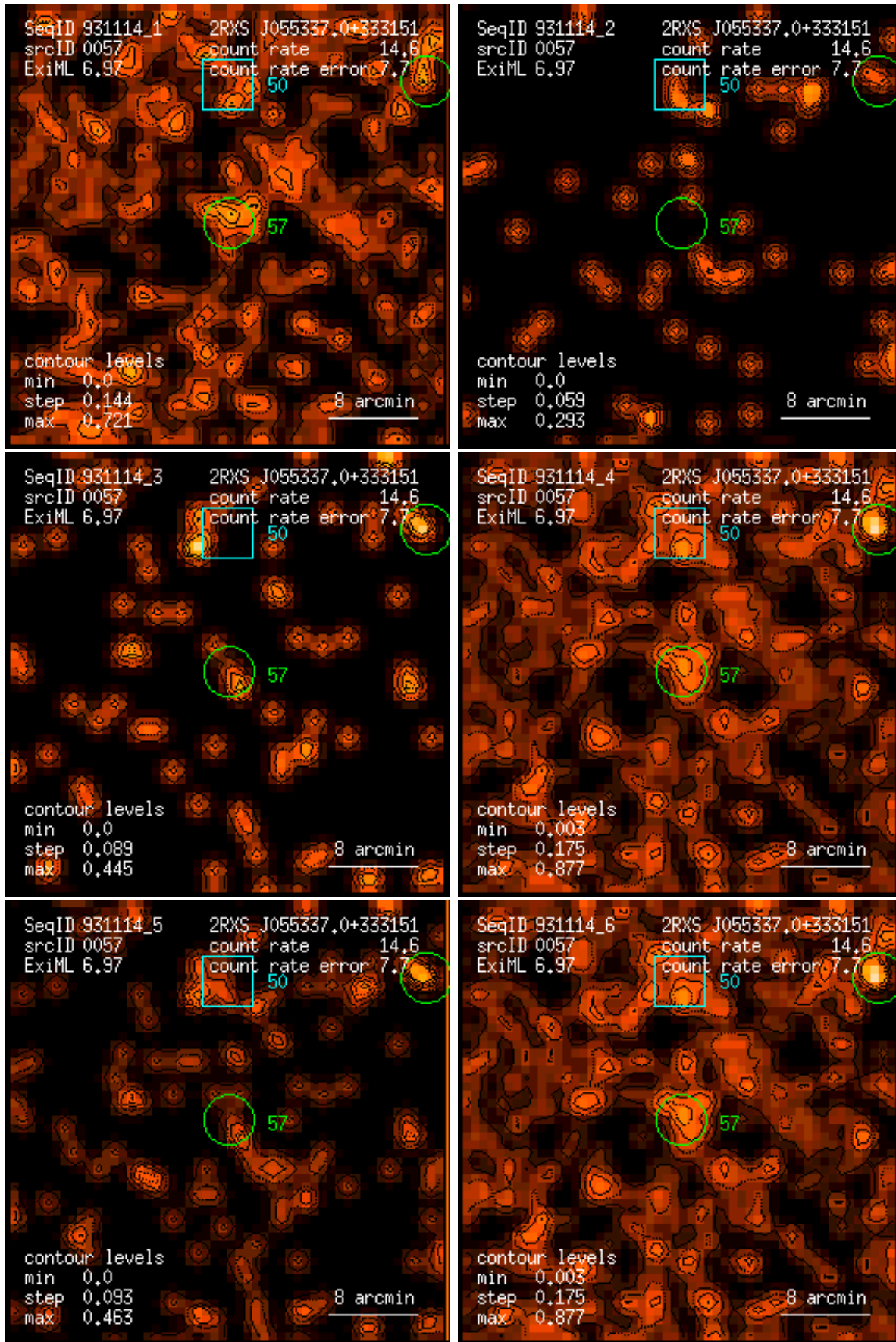
Figure 57: RASS 931114: detection 0057: band rate images, Gaussian filter: (1) PSPC channels 11 – 41, (2) 52 – 90, (3) 91 – 201, (4) 11 – 235, (5) 52 – 201, (6) 11 – 201. Broad band rates in counts/ks. Band rate contour levels in counts/ks/arcmin 2 .
