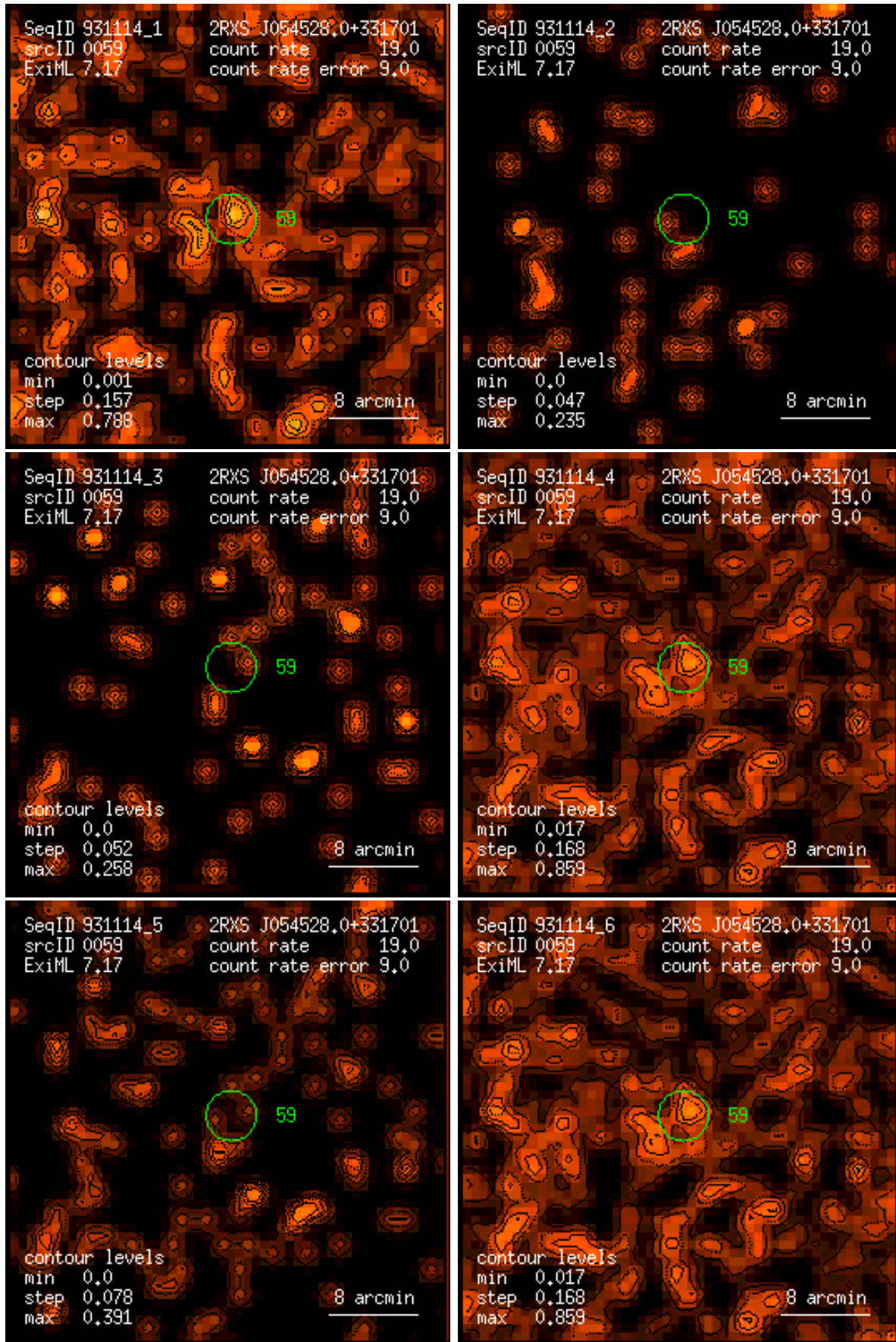
Figure 59: RASS 931114: detection 0059: band rate images, Gaussian filter: (1) PSPC channels 11 – 41, (2) 52 – 90, (3) 91 – 201, (4) 11 – 235, (5) 52 – 201, (6) 11 – 201. Broad band rates in counts/ks. Band rate contour levels in counts/ks/arcmin 2 .
