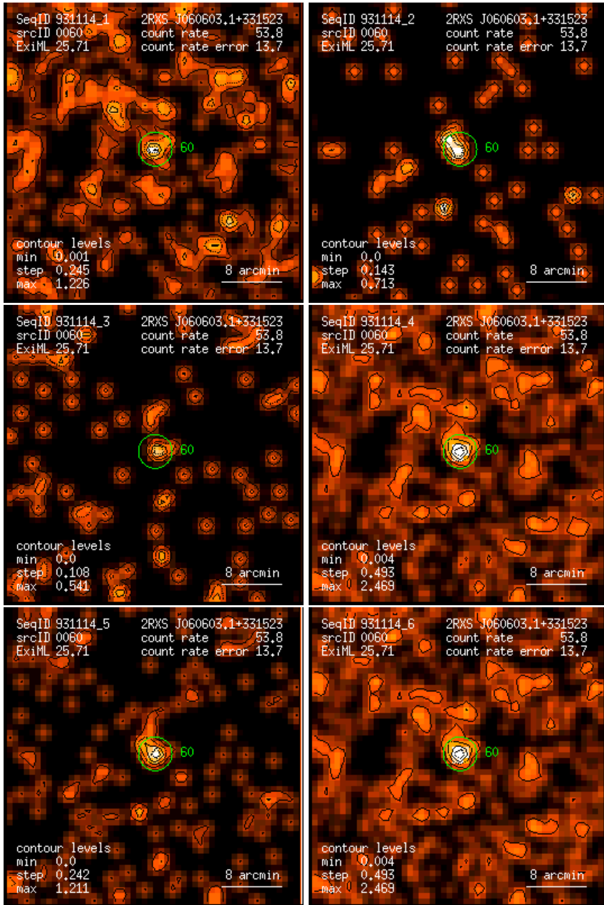
Figure 60: RASS 931114: detection 0060: band rate images, Gaussian filter: (1) PSPC channels 11 – 41, (2) 52 – 90, (3) 91 – 201, (4) 11 – 235, (5) 52 – 201, (6) 11 – 201. Broad band rates in counts/ks. Band rate contour levels in counts/ks/arcmin 2 .
