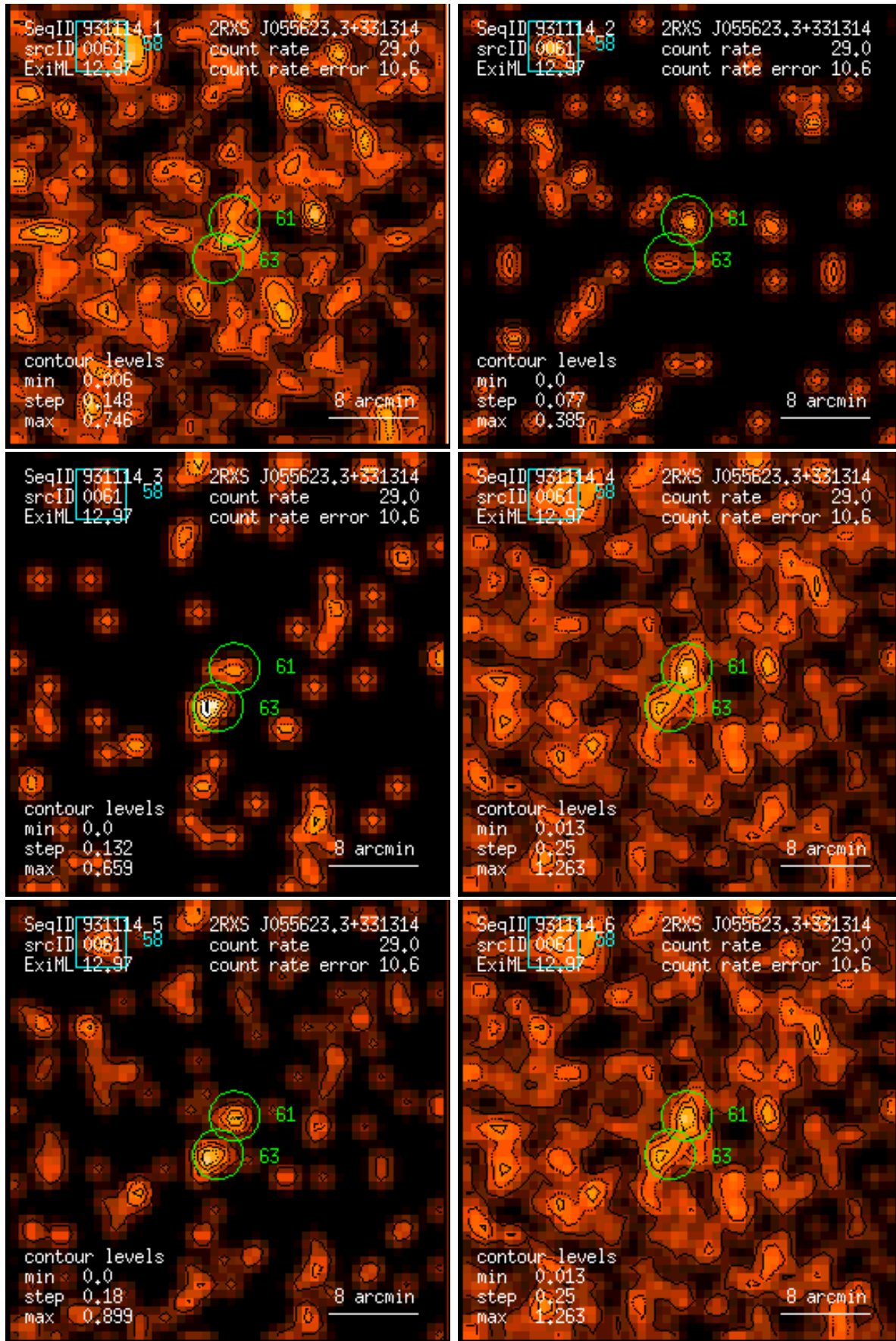
Figure 61: RASS 931114: detection 0061: band rate images, Gaussian filter: (1) PSPC channels 11 – 41, (2) 52 – 90, (3) 91 – 201, (4) 11 – 235, (5) 52 – 201, (6) 11 – 201. Broad band rates in counts/ks. Band rate contour levels in counts/ks/arcmin 2 .
