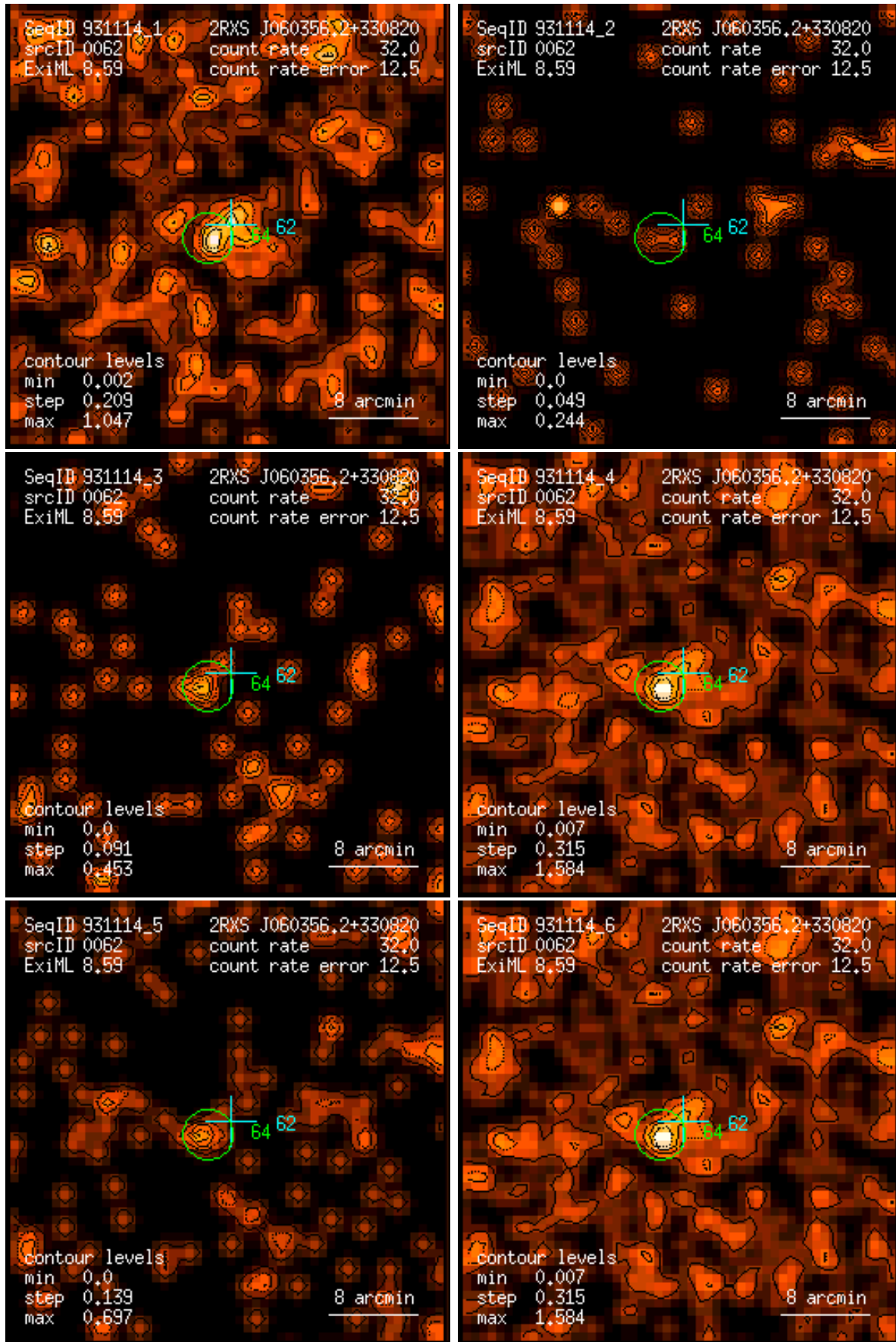
Figure 62: RASS 931114: detection 0062: band rate images, Gaussian filter: (1) PSPC channels 11 – 41, (2) 52 – 90, (3) 91 – 201, (4) 11 – 235, (5) 52 – 201, (6) 11 – 201. Broad band rates in counts/ks. Band rate contour levels in counts/ks/arcmin 2 .
