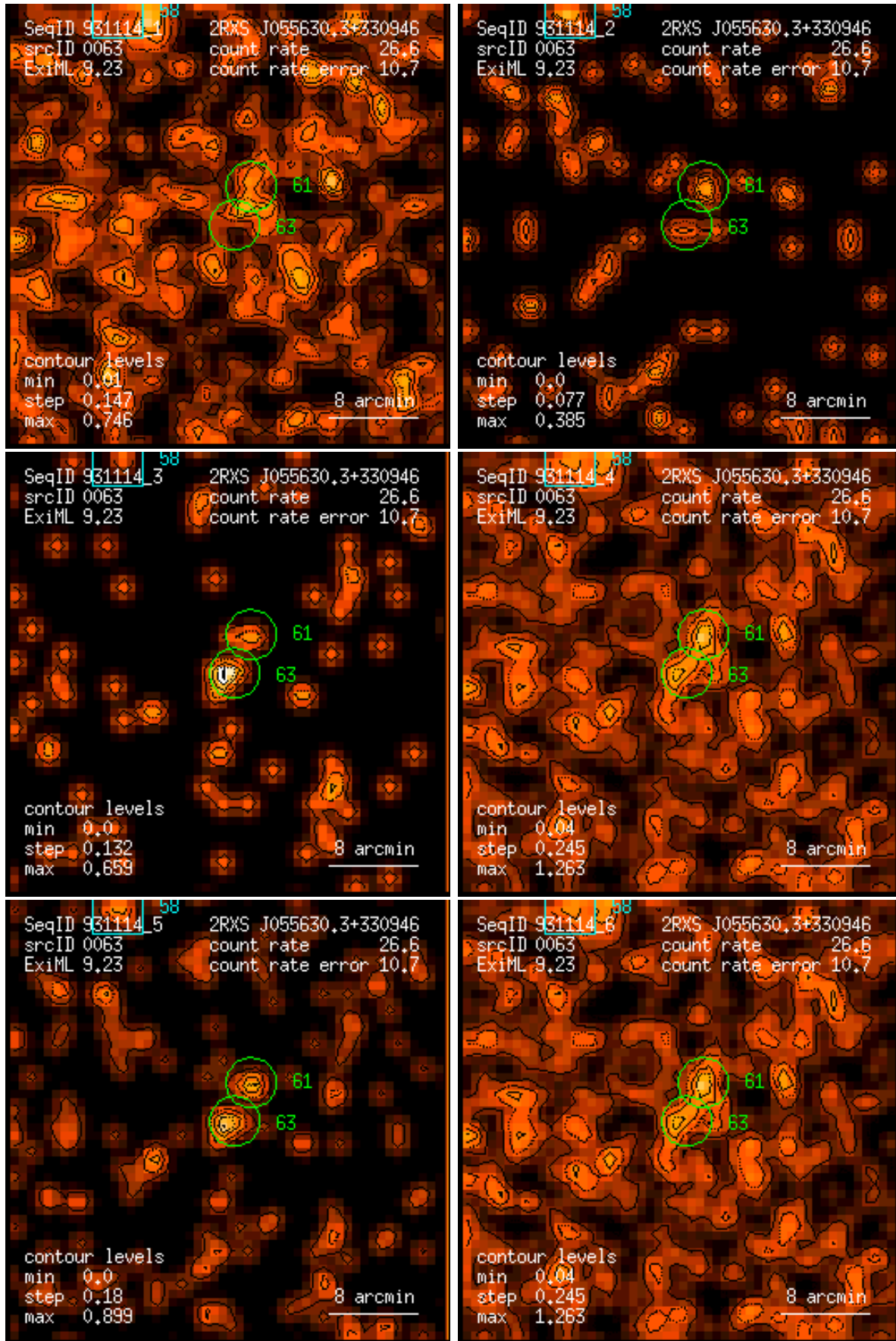
Figure 63: RASS 931114: detection 0063: band rate images, Gaussian filter: (1) PSPC channels 11 – 41, (2) 52 – 90, (3) 91 – 201, (4) 11 – 235, (5) 52 – 201, (6) 11 – 201. Broad band rates in counts/ks. Band rate contour levels in counts/ks/arcmin 2 .
