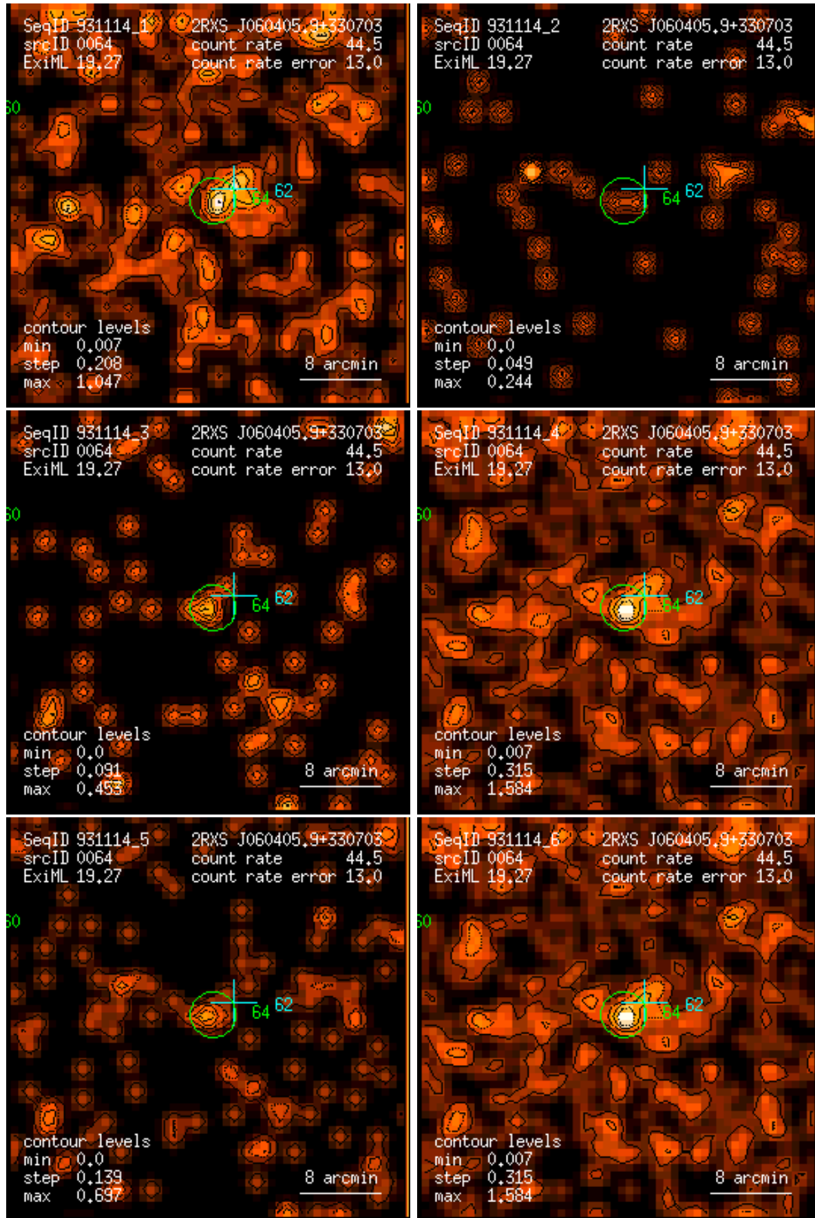
Figure 64: RASS 931114: detection 0064: band rate images, Gaussian filter: (1) PSPC channels 11 – 41, (2) 52 – 90, (3) 91 – 201, (4) 11 – 235, (5) 52 – 201, (6) 11 – 201. Broad band rates in counts/ks. Band rate contour levels in counts/ks/arcmin 2 .
