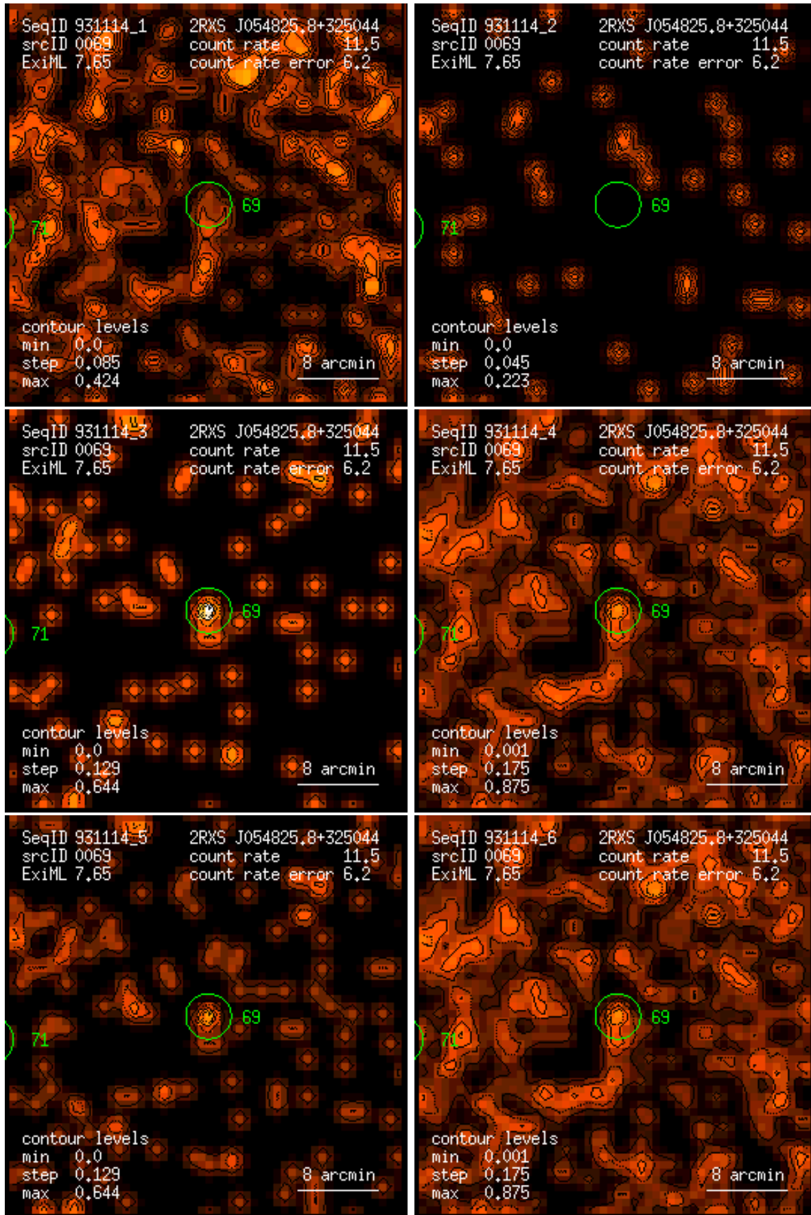
Figure 69: RASS 931114: detection 0069: band rate images, Gaussian filter: (1) PSPC channels 11 – 41, (2) 52 – 90, (3) 91 – 201, (4) 11 – 235, (5) 52 – 201, (6) 11 – 201. Broad band rates in counts/ks. Band rate contour levels in counts/ks/arcmin 2 .
