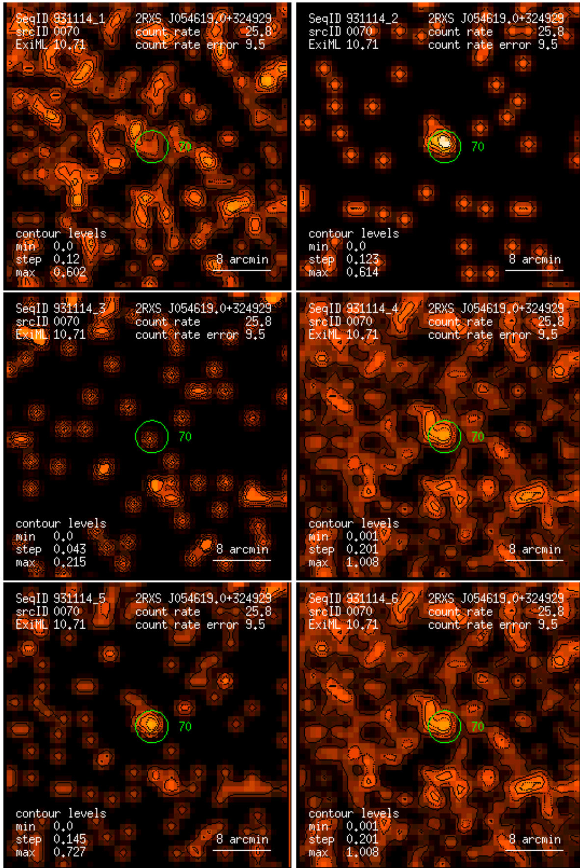
Figure 70: RASS 931114: detection 0070: band rate images, Gaussian filter: (1) PSPC channels 11 – 41, (2) 52 – 90, (3) 91 – 201, (4) 11 – 235, (5) 52 – 201, (6) 11 – 201. Broad band rates in counts/ks. Band rate contour levels in counts/ks/arcmin 2 .
