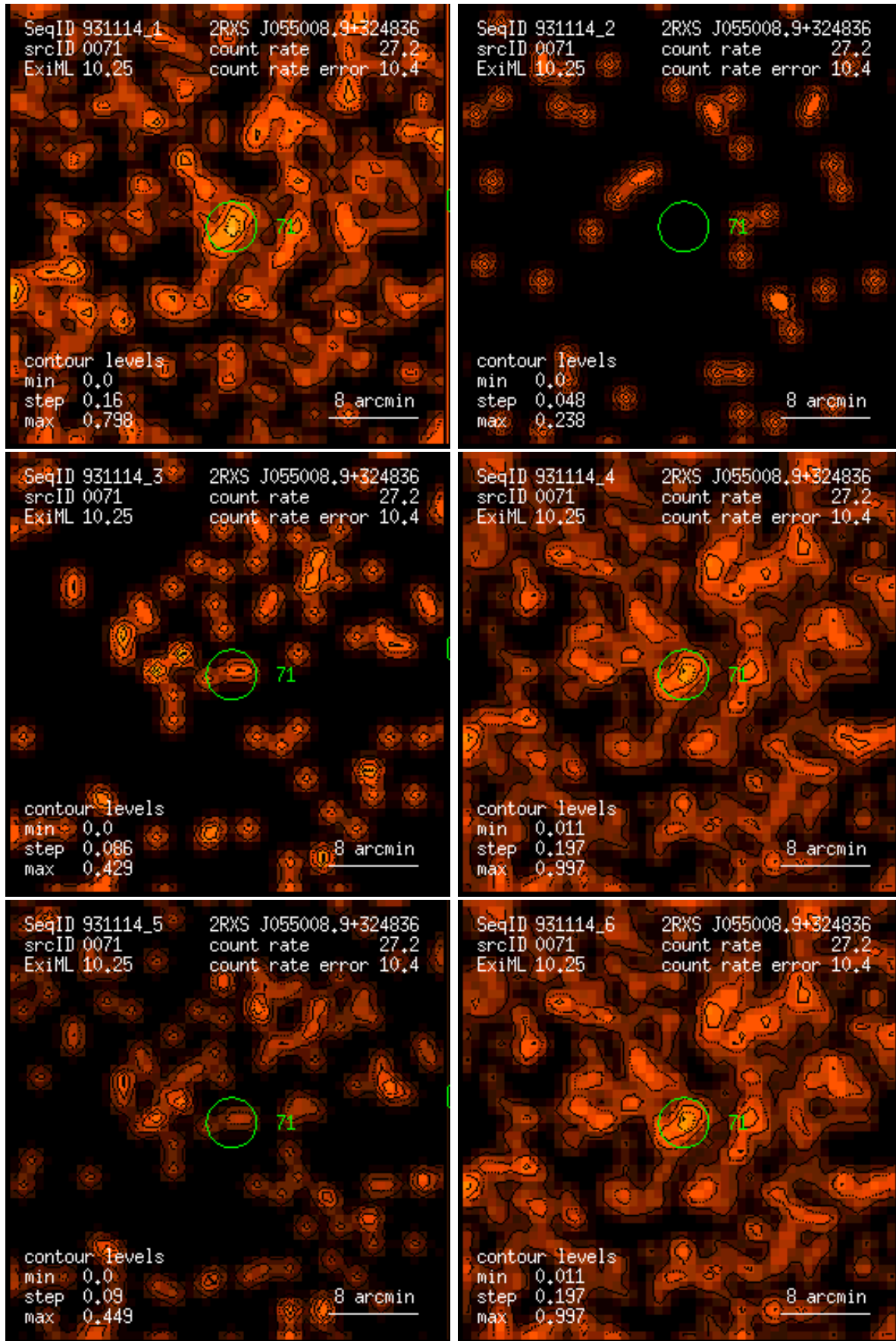
Figure 71: RASS 931114: detection 0071: band rate images, Gaussian filter: (1) PSPC channels 11 – 41, (2) 52 – 90, (3) 91 – 201, (4) 11 – 235, (5) 52 – 201, (6) 11 – 201. Broad band rates in counts/ks. Band rate contour levels in counts/ks/arcmin 2 .
