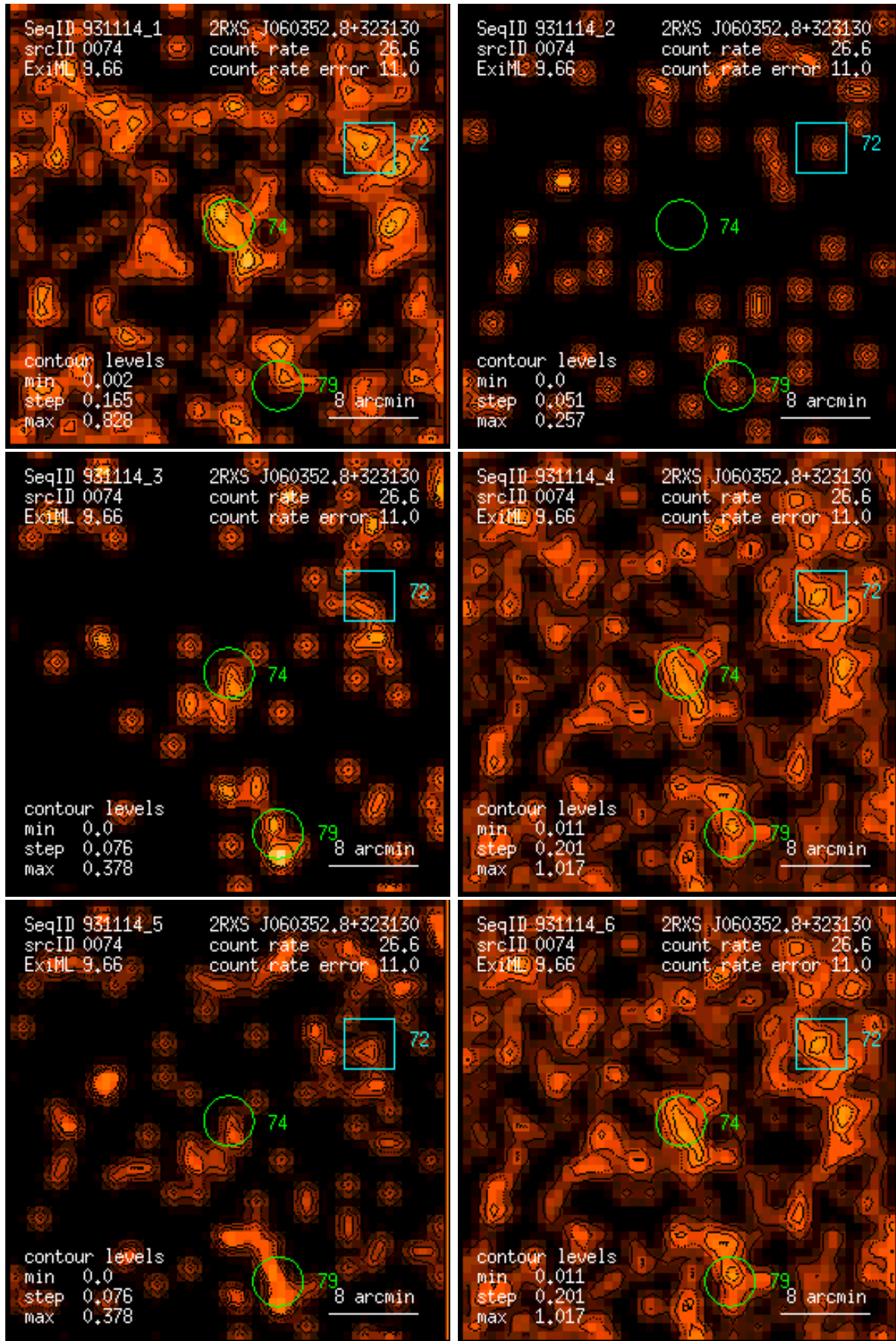
Figure 74: RASS 931114: detection 0074: band rate images, Gaussian filter: (1) PSPC channels 11 – 41, (2) 52 – 90, (3) 91 – 201, (4) 11 – 235, (5) 52 – 201, (6) 11 – 201. Broad band rates in counts/ks. Band rate contour levels in counts/ks/arcmin 2 .
