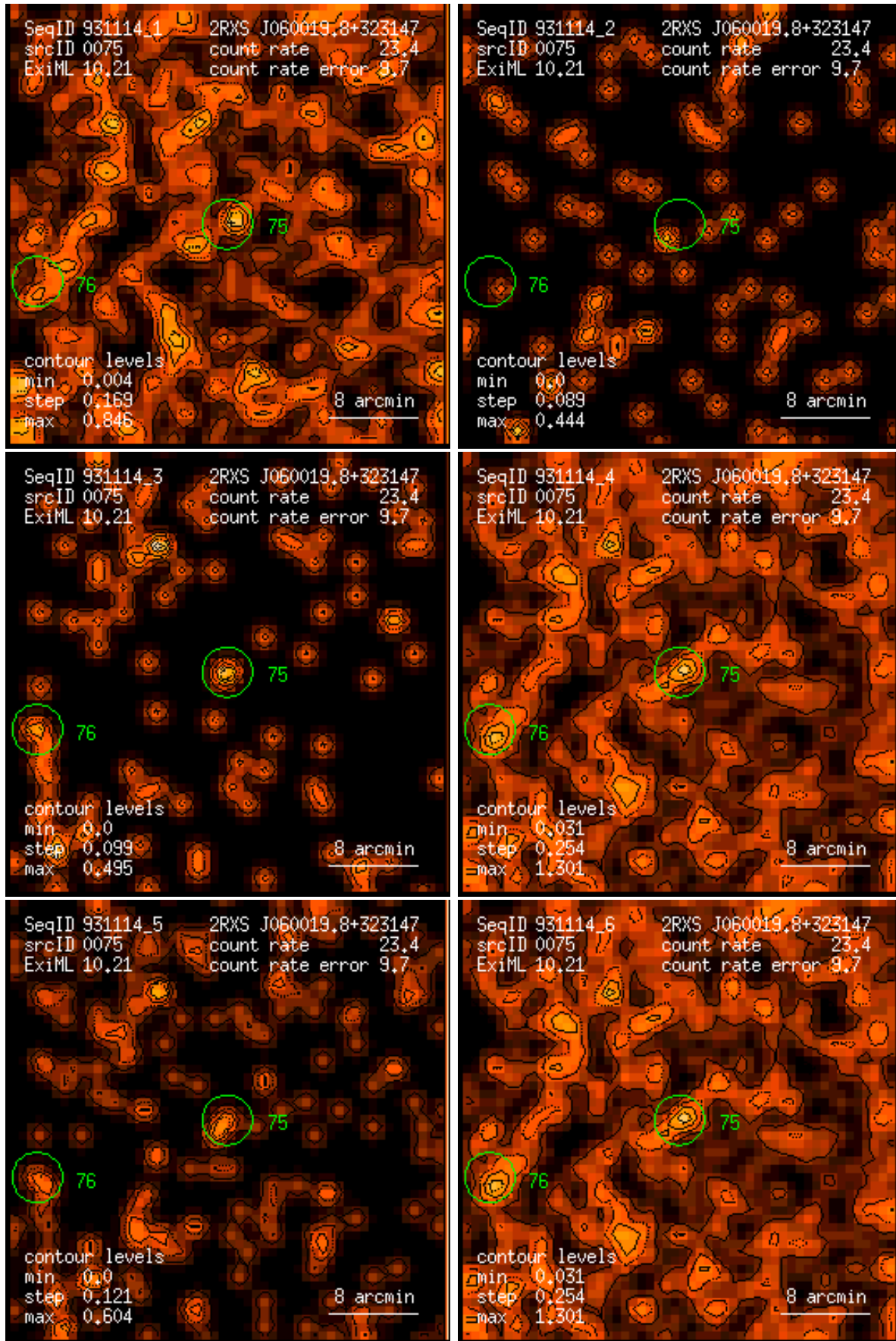
Figure 75: RASS 931114: detection 0075: band rate images, Gaussian filter: (1) PSPC channels 11 – 41, (2) 52 – 90, (3) 91 – 201, (4) 11 – 235, (5) 52 – 201, (6) 11 – 201. Broad band rates in counts/ks. Band rate contour levels in counts/ks/arcmin 2 .
