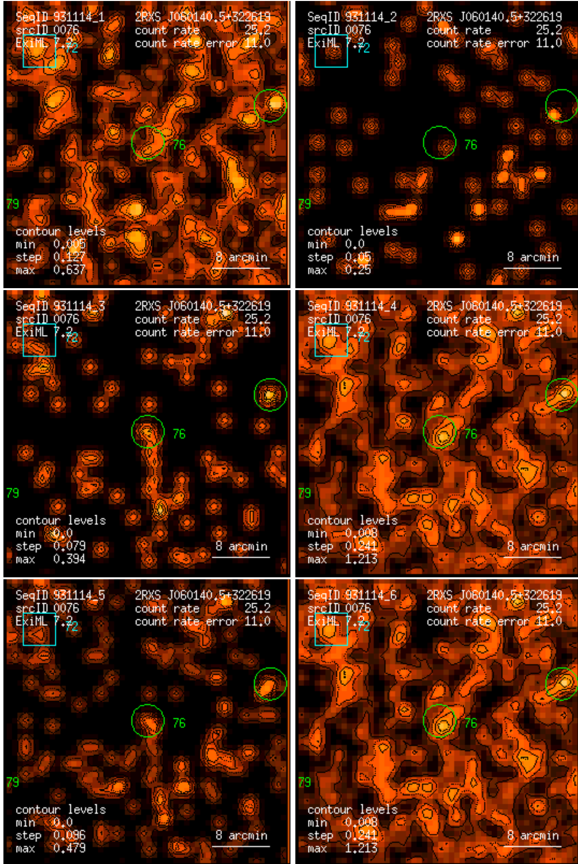
Figure 76: RASS 931114: detection 0076: band rate images, Gaussian filter: (1) PSPC channels 11 – 41, (2) 52 – 90, (3) 91 – 201, (4) 11 – 235, (5) 52 – 201, (6) 11 – 201. Broad band rates in counts/ks. Band rate contour levels in counts/ks/arcmin 2 .
