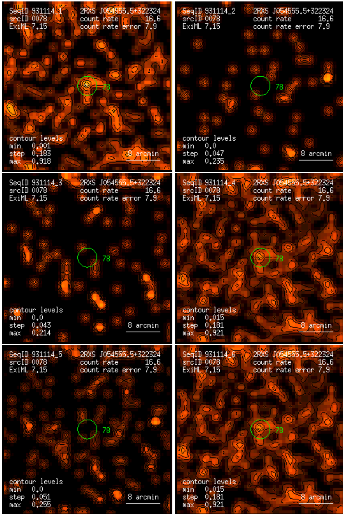
Figure 78: RASS 931114: detection 0078: band rate images, Gaussian filter: (1) PSPC channels 11 – 41, (2) 52 – 90, (3) 91 – 201, (4) 11 – 235, (5) 52 – 201, (6) 11 – 201. Broad band rates in counts/ks. Band rate contour levels in counts/ks/arcmin 2 .
