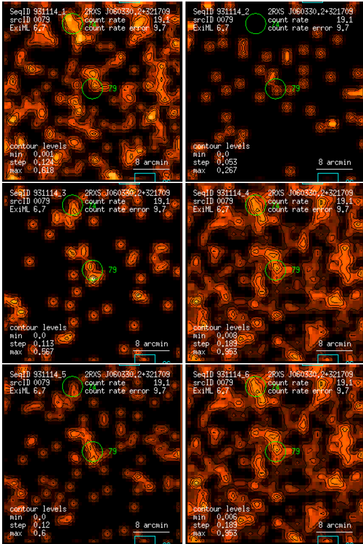
Figure 79: RASS 931114: detection 0079: band rate images, Gaussian filter: (1) PSPC channels 11 – 41, (2) 52 – 90, (3) 91 – 201, (4) 11 – 235, (5) 52 – 201, (6) 11 – 201. Broad band rates in counts/ks. Band rate contour levels in counts/ks/arcmin 2 .
