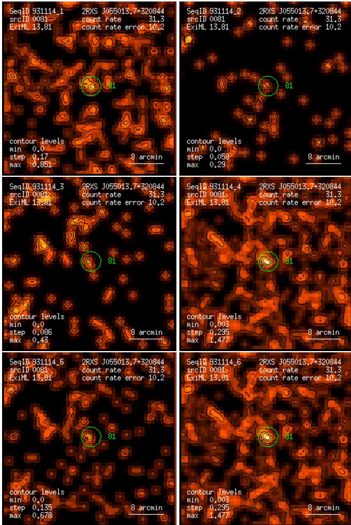
Figure 81: RASS 931114: detection 0081: band rate images, Gaussian filter: (1) PSPC channels 11 – 41, (2) 52 – 90, (3) 91 – 201, (4) 11 – 235, (5) 52 – 201, (6) 11 – 201. Broad band rates in counts/ks. Band rate contour levels in counts/ks/arcmin 2 .
