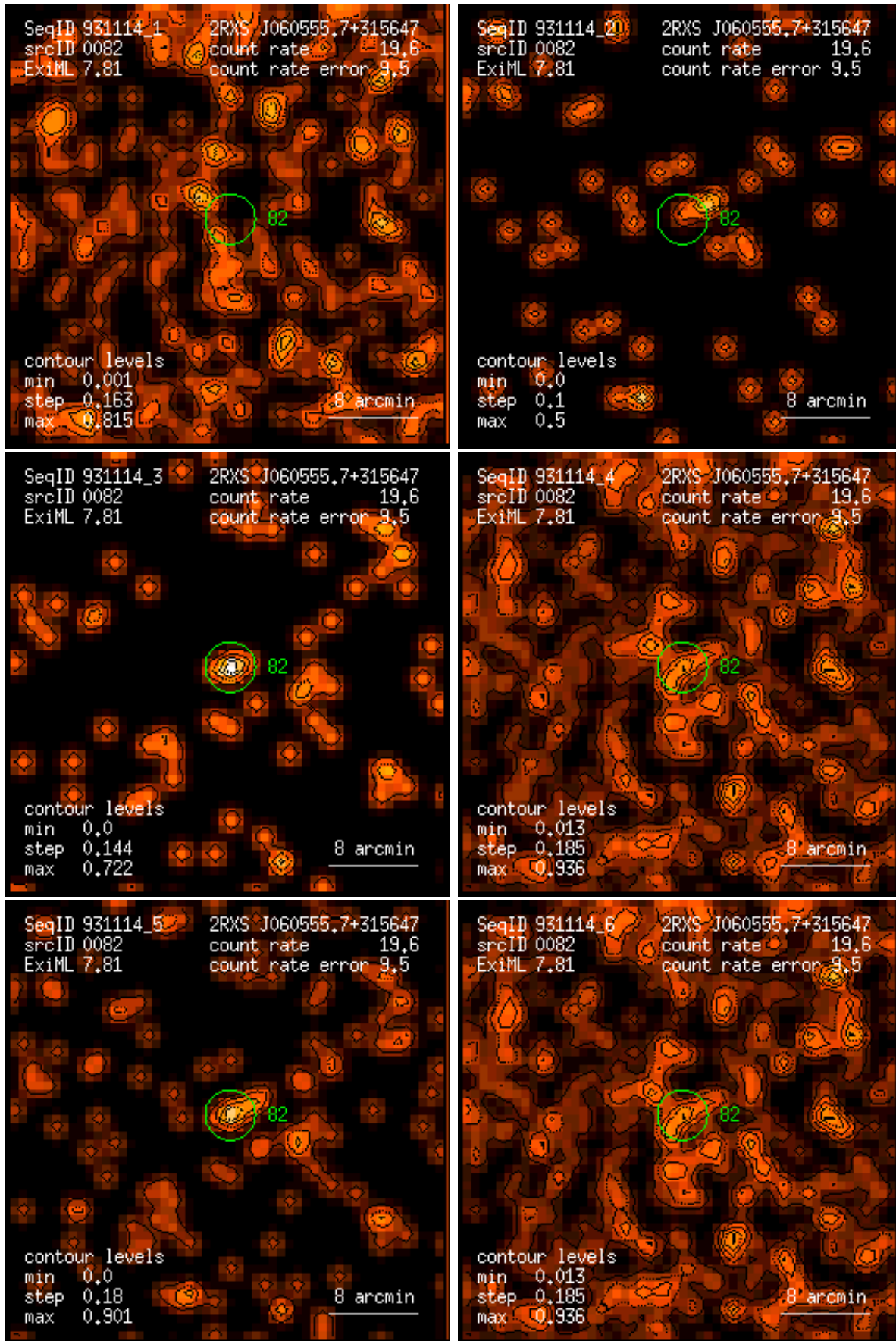
Figure 82: RASS 931114: detection 0082: band rate images, Gaussian filter: (1) PSPC channels 11 – 41, (2) 52 – 90, (3) 91 – 201, (4) 11 – 235, (5) 52 – 201, (6) 11 – 201. Broad band rates in counts/ks. Band rate contour levels in counts/ks/arcmin 2 .
