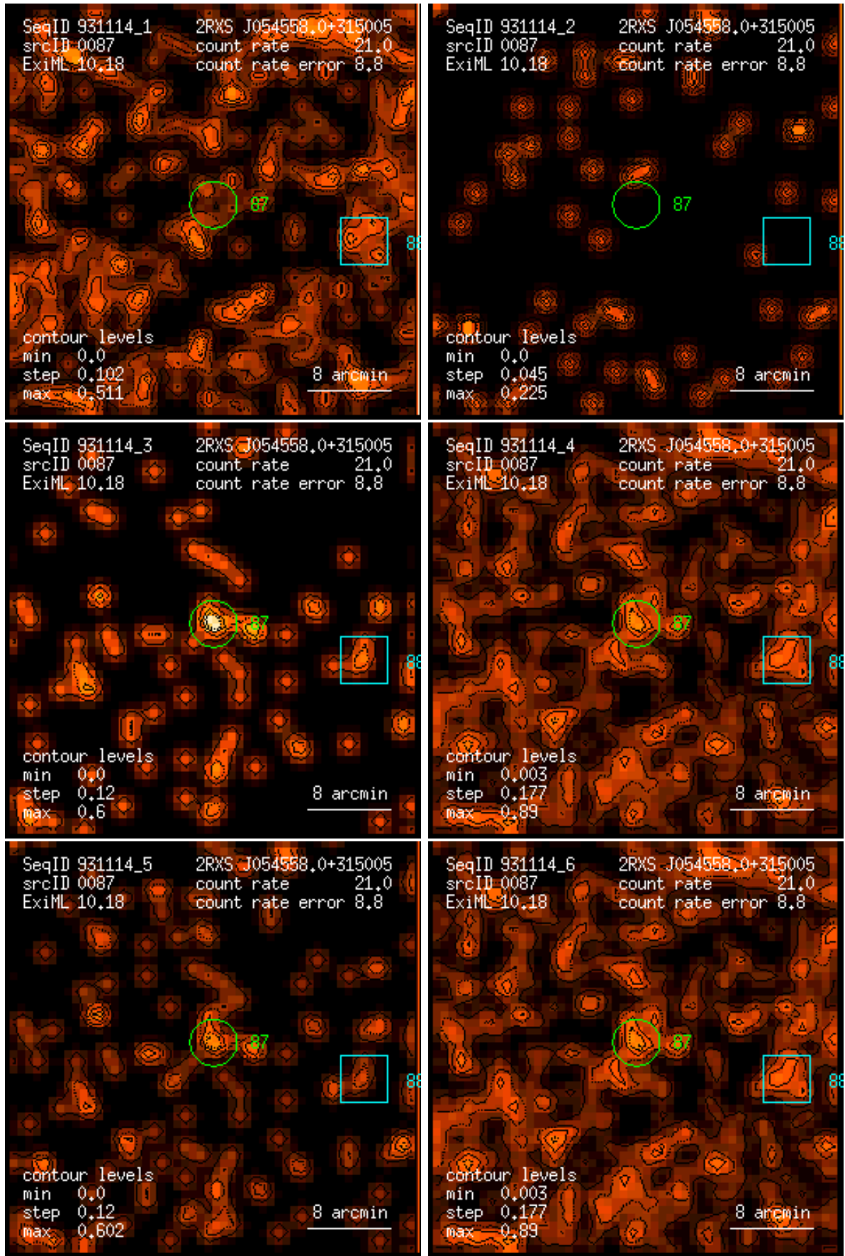
Figure 87: RASS 931114: detection 0087: band rate images, Gaussian filter: (1) PSPC channels 11 – 41, (2) 52 – 90, (3) 91 – 201, (4) 11 – 235, (5) 52 – 201, (6) 11 – 201. Broad band rates in counts/ks. Band rate contour levels in counts/ks/arcmin 2 .
