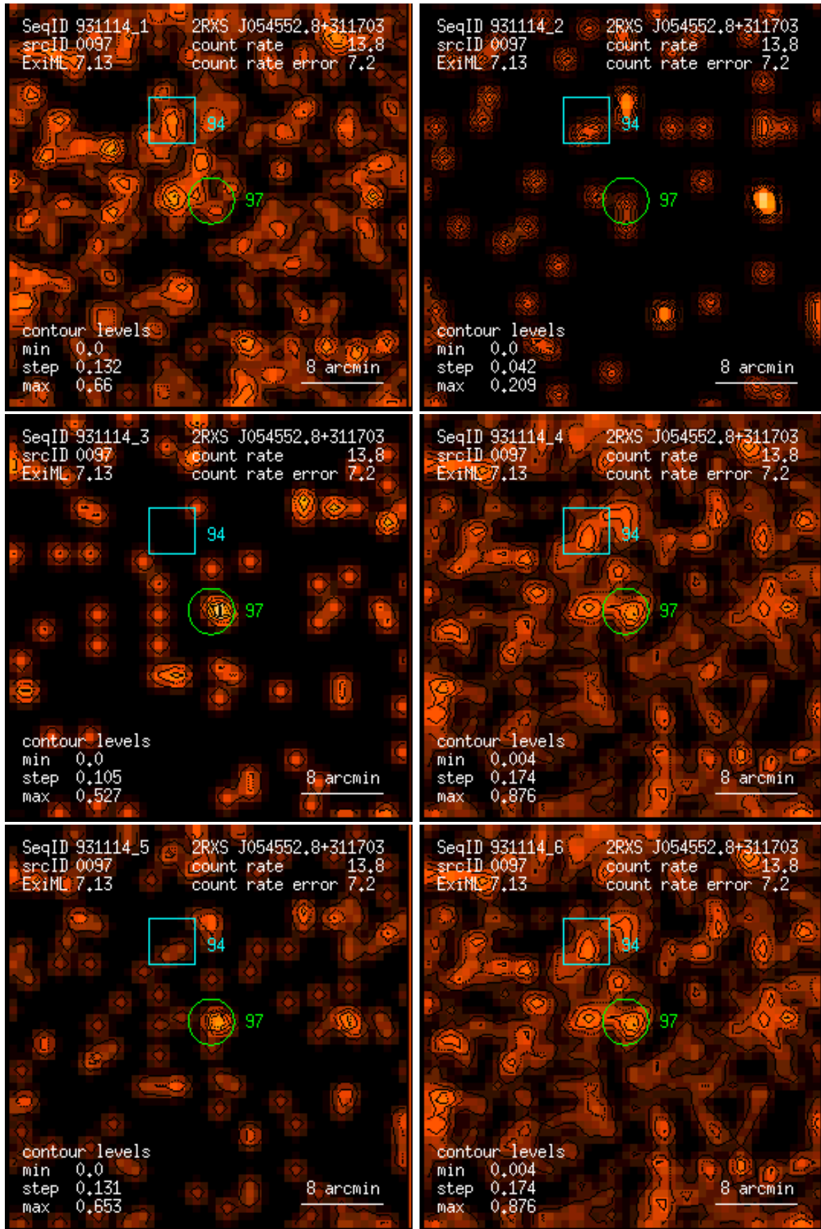
Figure 97: RASS 931114: detection 0097: band rate images, Gaussian filter: (1) PSPC channels 11 – 41, (2) 52 – 90, (3) 91 – 201, (4) 11 – 235, (5) 52 – 201, (6) 11 – 201. Broad band rates in counts/ks. Band rate contour levels in counts/ks/arcmin 2 .
