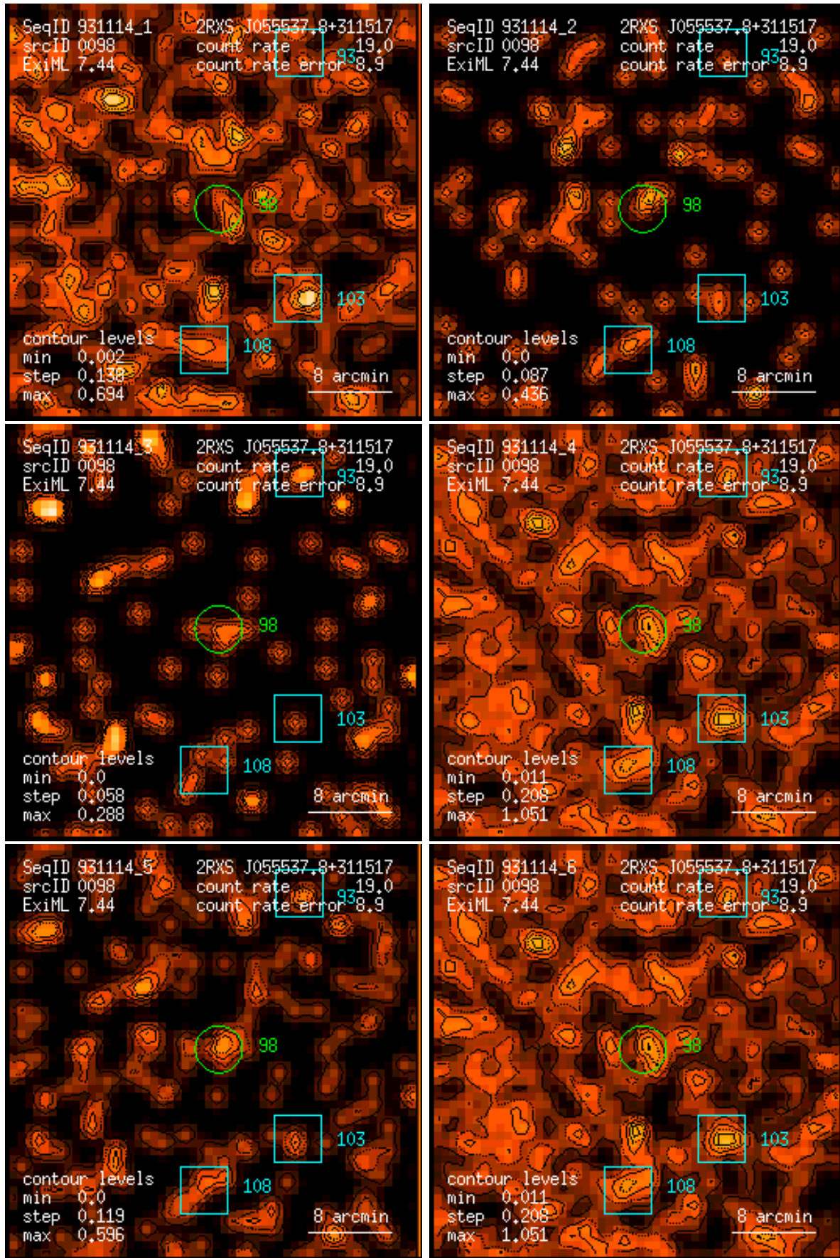
Figure 98: RASS 931114: detection 0098: band rate images, Gaussian filter: (1) PSPC channels 11 – 41, (2) 52 – 90, (3) 91 – 201, (4) 11 – 235, (5) 52 – 201, (6) 11 – 201. Broad band rates in counts/ks. Band rate contour levels in counts/ks/arcmin 2 .
