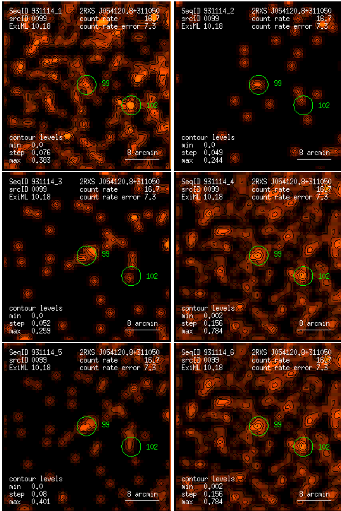
Figure 99: RASS 931114: detection 0099: band rate images, Gaussian filter: (1) PSPC channels 11 – 41, (2) 52 – 90, (3) 91 – 201, (4) 11 – 235, (5) 52 – 201, (6) 11 – 201. Broad band rates in counts/ks. Band rate contour levels in counts/ks/arcmin 2 .
