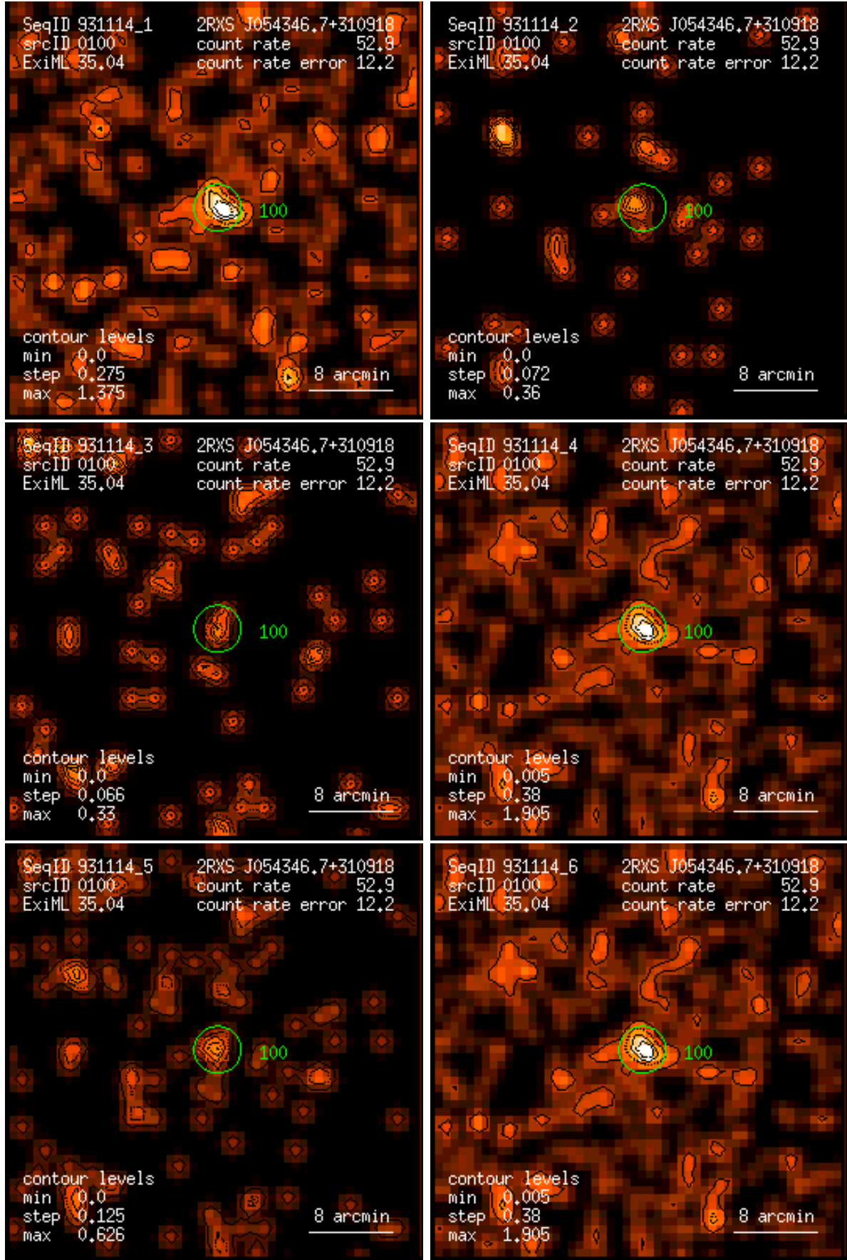
Figure 100: RASS 931114: detection 0100: band rate images, Gaussian filter: (1) PSPC channels 11 – 41, (2) 52 – 90, (3) 91 – 201, (4) 11 – 235, (5) 52 – 201, (6) 11 – 201. Broad band rates in counts/ks. Band rate contour levels in counts/ks/arcmin 2 .
