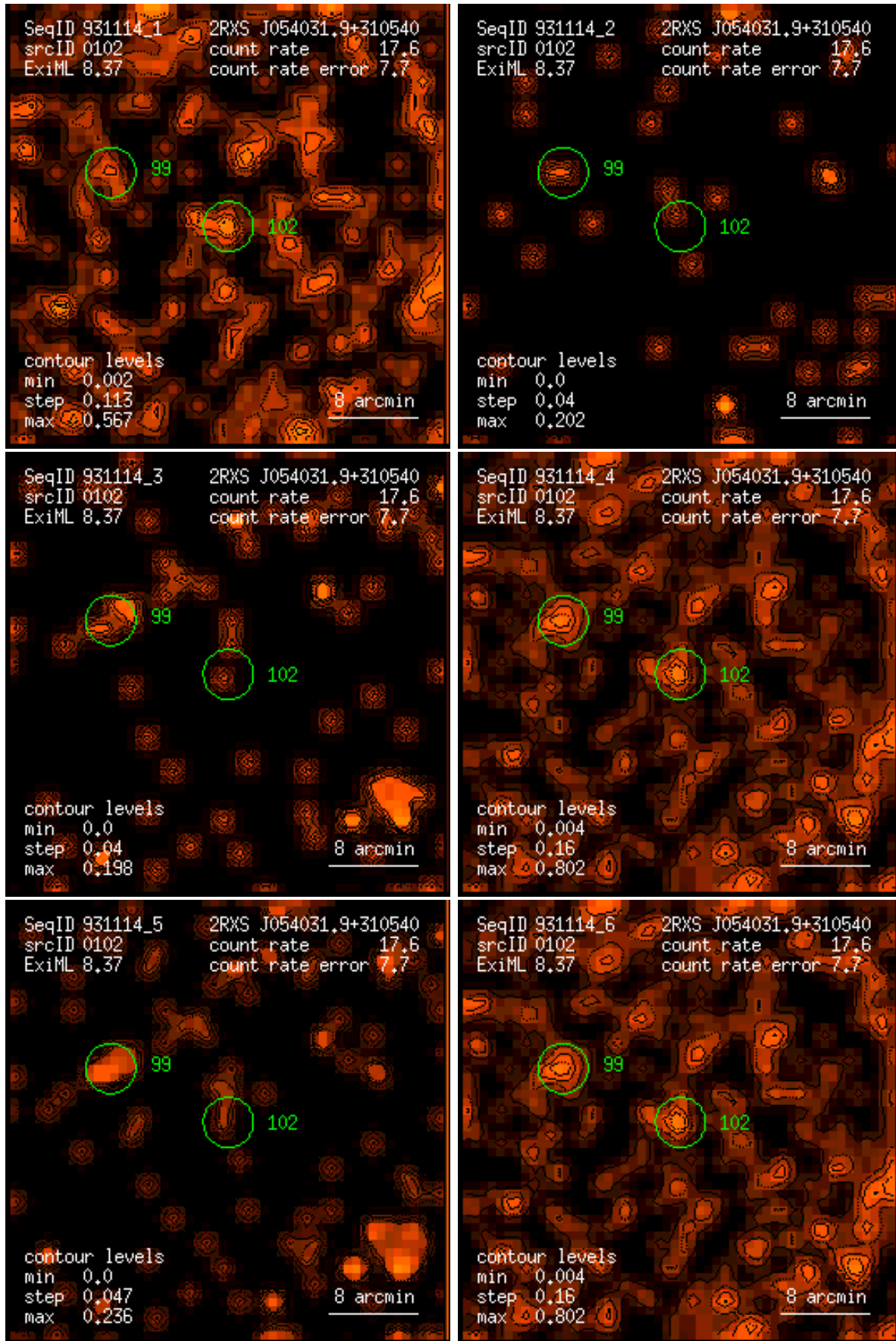
Figure 102: RASS 931114: detection 0102: band rate images, Gaussian filter: (1) PSPC channels 11 – 41, (2) 52 – 90, (3) 91 – 201, (4) 11 – 235, (5) 52 – 201, (6) 11 – 201. Broad band rates in counts/ks. Band rate contour levels in counts/ks/arcmin 2 .
