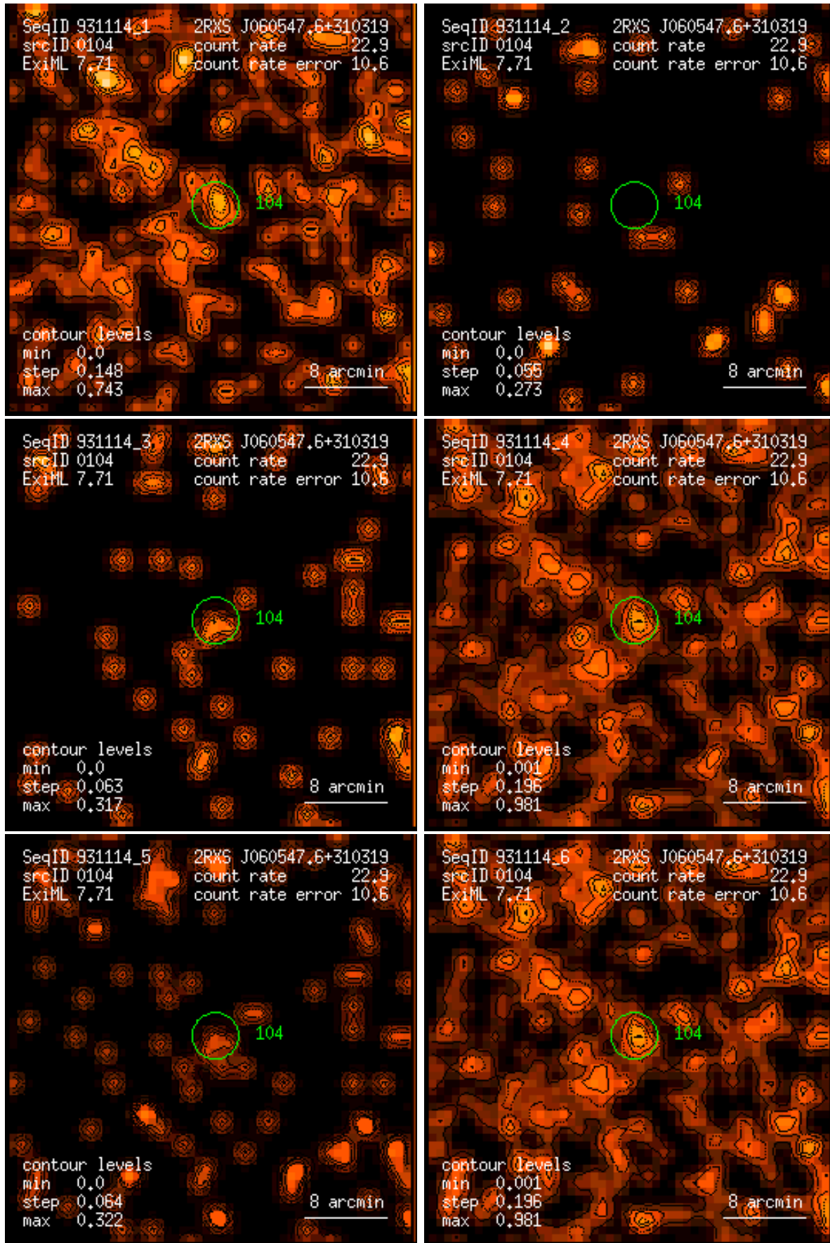
Figure 104: RASS 931114: detection 0104: band rate images, Gaussian filter: (1) PSPC channels 11 – 41, (2) 52 – 90, (3) 91 – 201, (4) 11 – 235, (5) 52 – 201, (6) 11 – 201. Broad band rates in counts/ks. Band rate contour levels in counts/ks/arcmin 2 .
