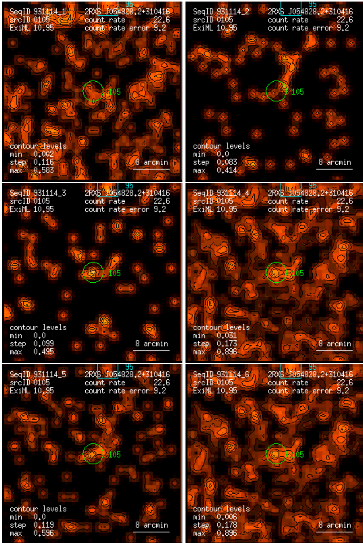
Figure 105: RASS 931114: detection 0105: band rate images, Gaussian filter: (1) PSPC channels 11 – 41, (2) 52 – 90, (3) 91 – 201, (4) 11 – 235, (5) 52 – 201, (6) 11 – 201. Broad band rates in counts/ks. Band rate contour levels in counts/ks/arcmin 2 .
