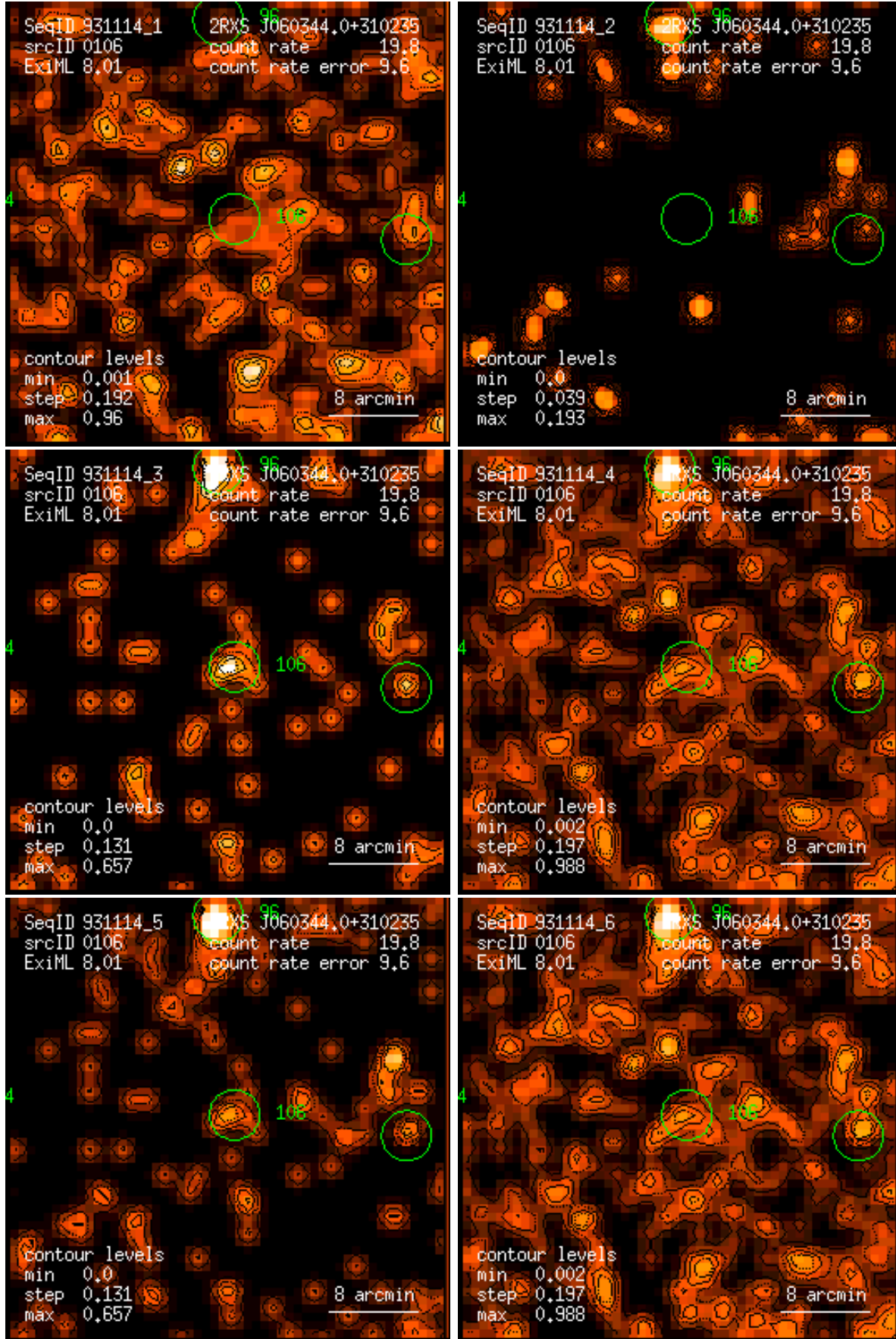
Figure 106: RASS 931114: detection 0106: band rate images, Gaussian filter: (1) PSPC channels 11 – 41, (2) 52 – 90, (3) 91 – 201, (4) 11 – 235, (5) 52 – 201, (6) 11 – 201. Broad band rates in counts/ks. Band rate contour levels in counts/ks/arcmin 2 .
