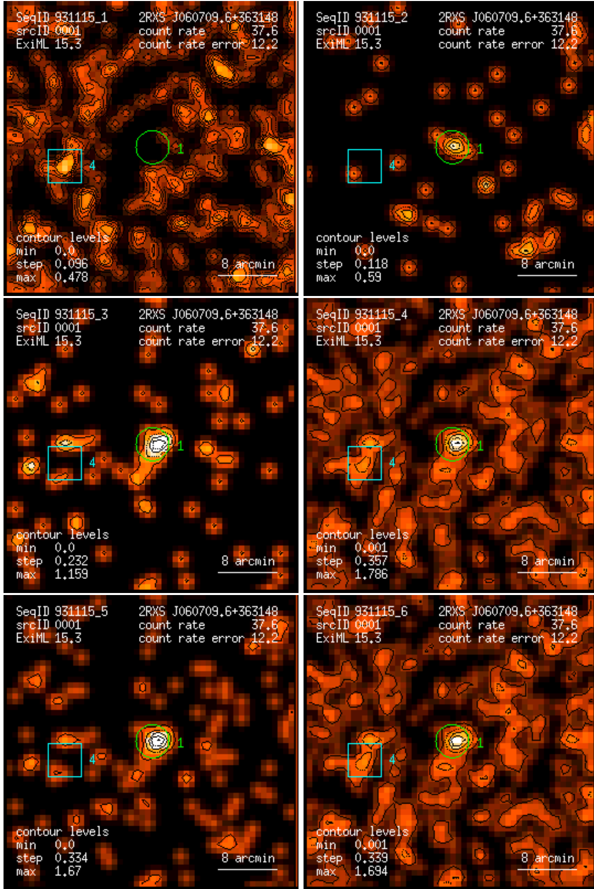
Figure 1: RASS 931115: detection 0001: band rate images, Gaussian filter: (1) PSPC channels 11 – 41, (2) 52 – 90, (3) 91 – 201, (4) 11 – 235, (5) 52 – 201, (6) 11 – 201. Broad band rates in counts/ks. Band rate contour levels in counts/ks/arcmin 2 .
