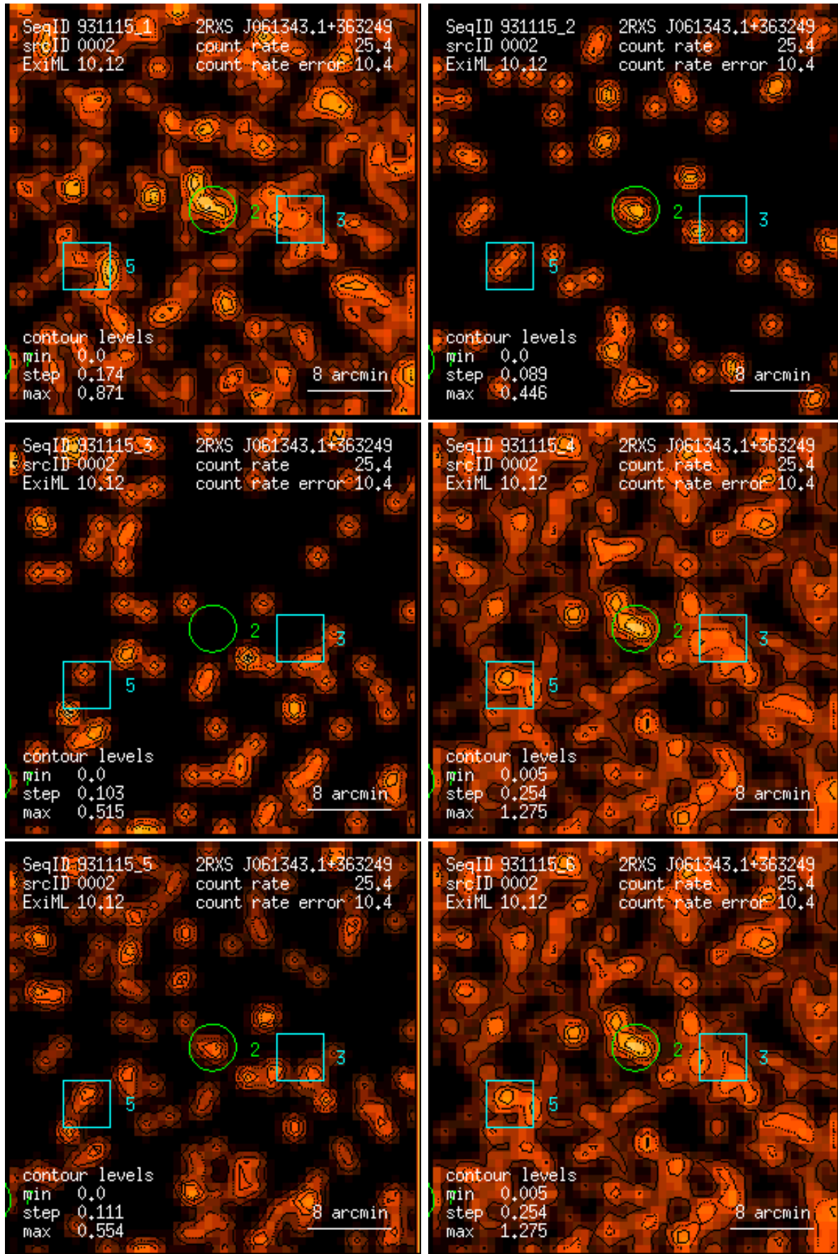
Figure 2: RASS 931115: detection 0002: band rate images, Gaussian filter: (1) PSPC channels 11 – 41, (2) 52 – 90, (3) 91 – 201, (4) 11 – 235, (5) 52 – 201, (6) 11 – 201. Broad band rates in counts/ks. Band rate contour levels in counts/ks/arcmin 2 .
