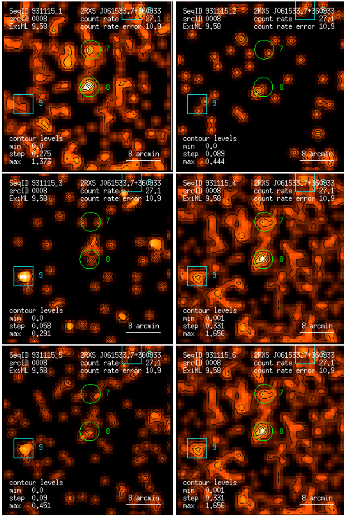
Figure 8: RASS 931115: detection 0008: band rate images, Gaussian filter: (1) PSPC channels 11 – 41, (2) 52 – 90, (3) 91 – 201, (4) 11 – 235, (5) 52 – 201, (6) 11 – 201. Broad band rates in counts/ks. Band rate contour levels in counts/ks/arcmin 2 .
