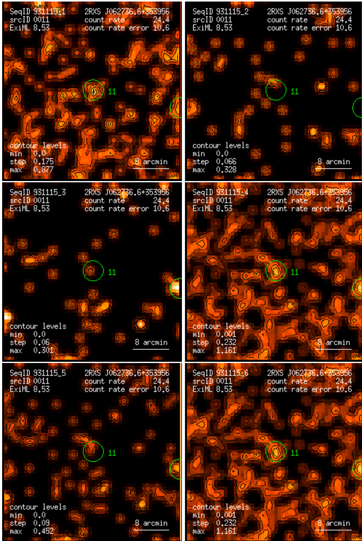
Figure 11: RASS 931115: detection 0011: band rate images, Gaussian filter: (1) PSPC channels 11 – 41, (2) 52 – 90, (3) 91 – 201, (4) 11 – 235, (5) 52 – 201, (6) 11 – 201. Broad band rates in counts/ks. Band rate contour levels in counts/ks/arcmin 2 .
