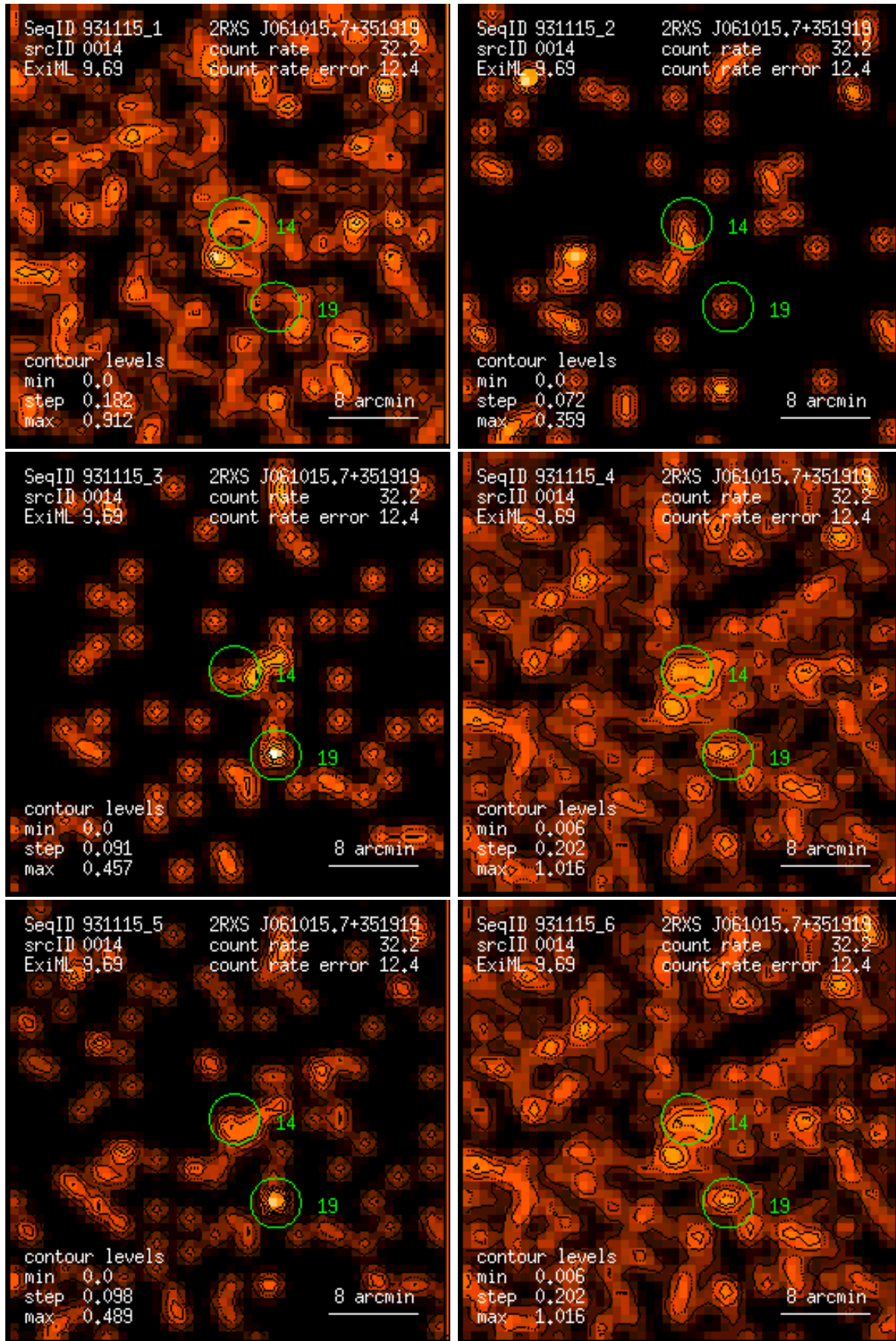
Figure 14: RASS 931115: detection 0014: band rate images, Gaussian filter: (1) PSPC channels 11 – 41, (2) 52 – 90, (3) 91 – 201, (4) 11 – 235, (5) 52 – 201, (6) 11 – 201. Broad band rates in counts/ks. Band rate contour levels in counts/ks/arcmin 2 .
