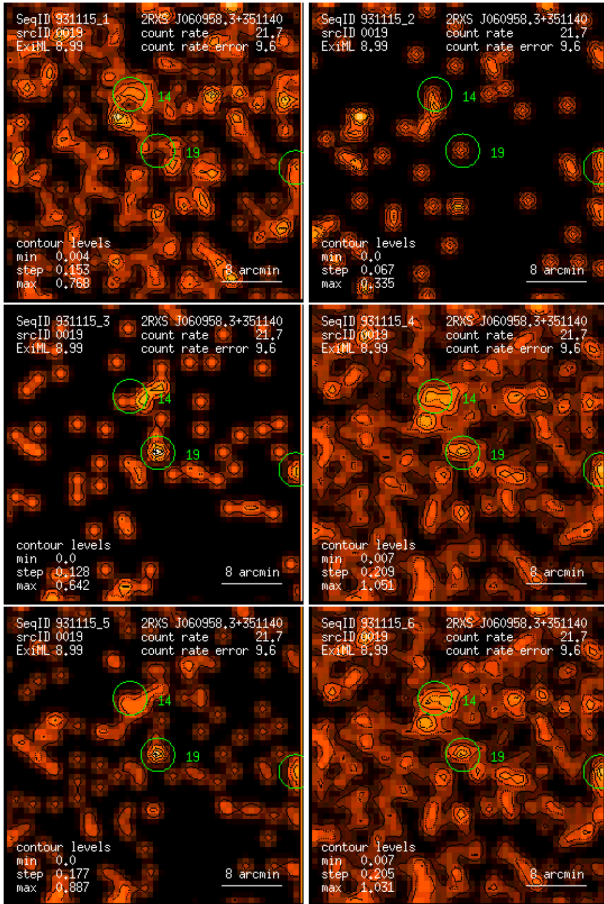
Figure 19: RASS 931115: detection 0019: band rate images, Gaussian filter: (1) PSPC channels 11 – 41, (2) 52 – 90, (3) 91 – 201, (4) 11 – 235, (5) 52 – 201, (6) 11 – 201. Broad band rates in counts/ks. Band rate contour levels in counts/ks/arcmin 2 .
