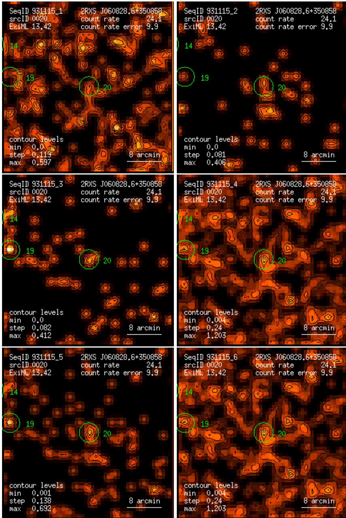
Figure 20: RASS 931115: detection 0020: band rate images, Gaussian filter: (1) PSPC channels 11 – 41, (2) 52 – 90, (3) 91 – 201, (4) 11 – 235, (5) 52 – 201, (6) 11 – 201. Broad band rates in counts/ks. Band rate contour levels in counts/ks/arcmin 2 .
