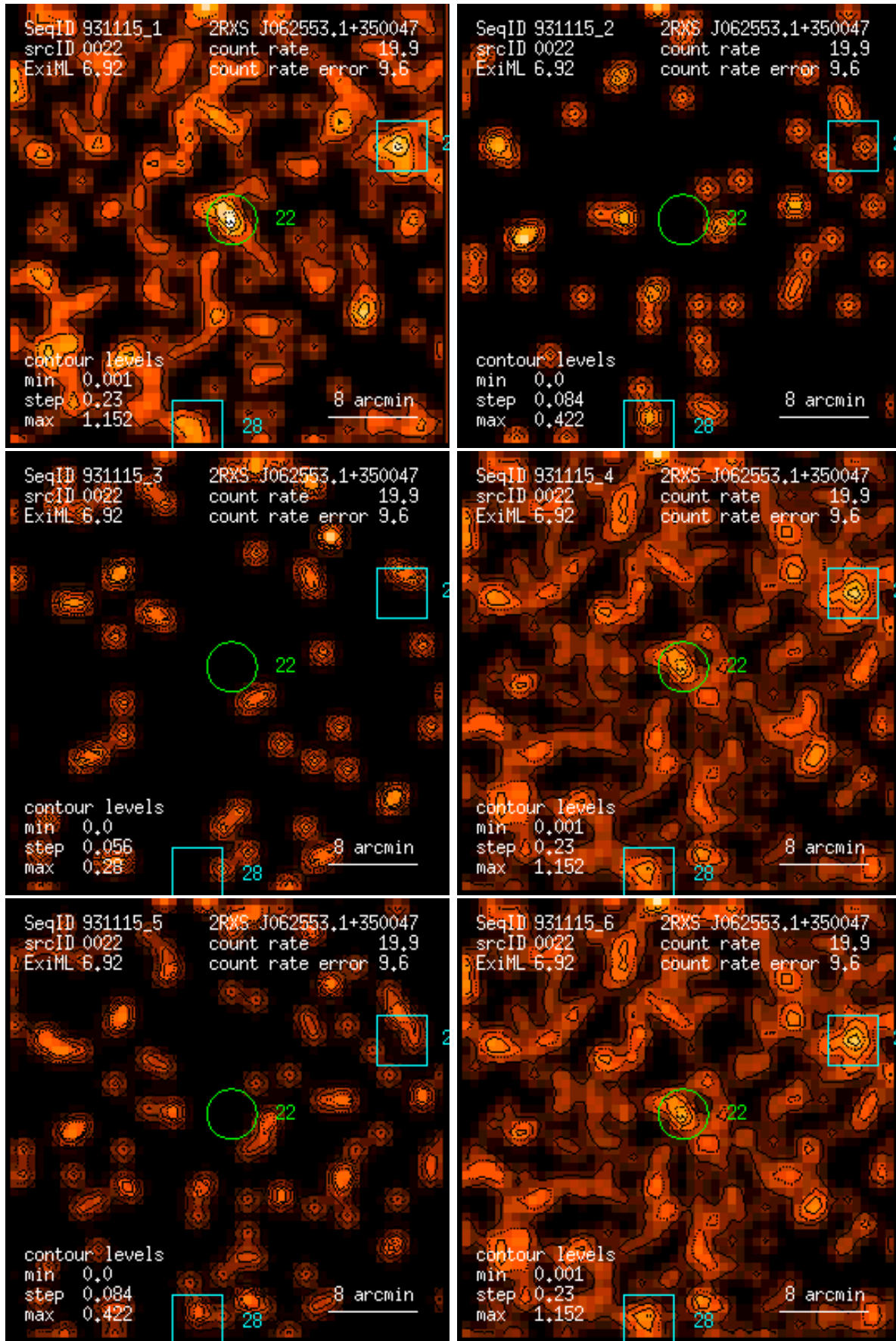
Figure 22: RASS 931115: detection 0022: band rate images, Gaussian filter: (1) PSPC channels 11 – 41, (2) 52 – 90, (3) 91 – 201, (4) 11 – 235, (5) 52 – 201, (6) 11 – 201. Broad band rates in counts/ks. Band rate contour levels in counts/ks/arcmin 2 .
