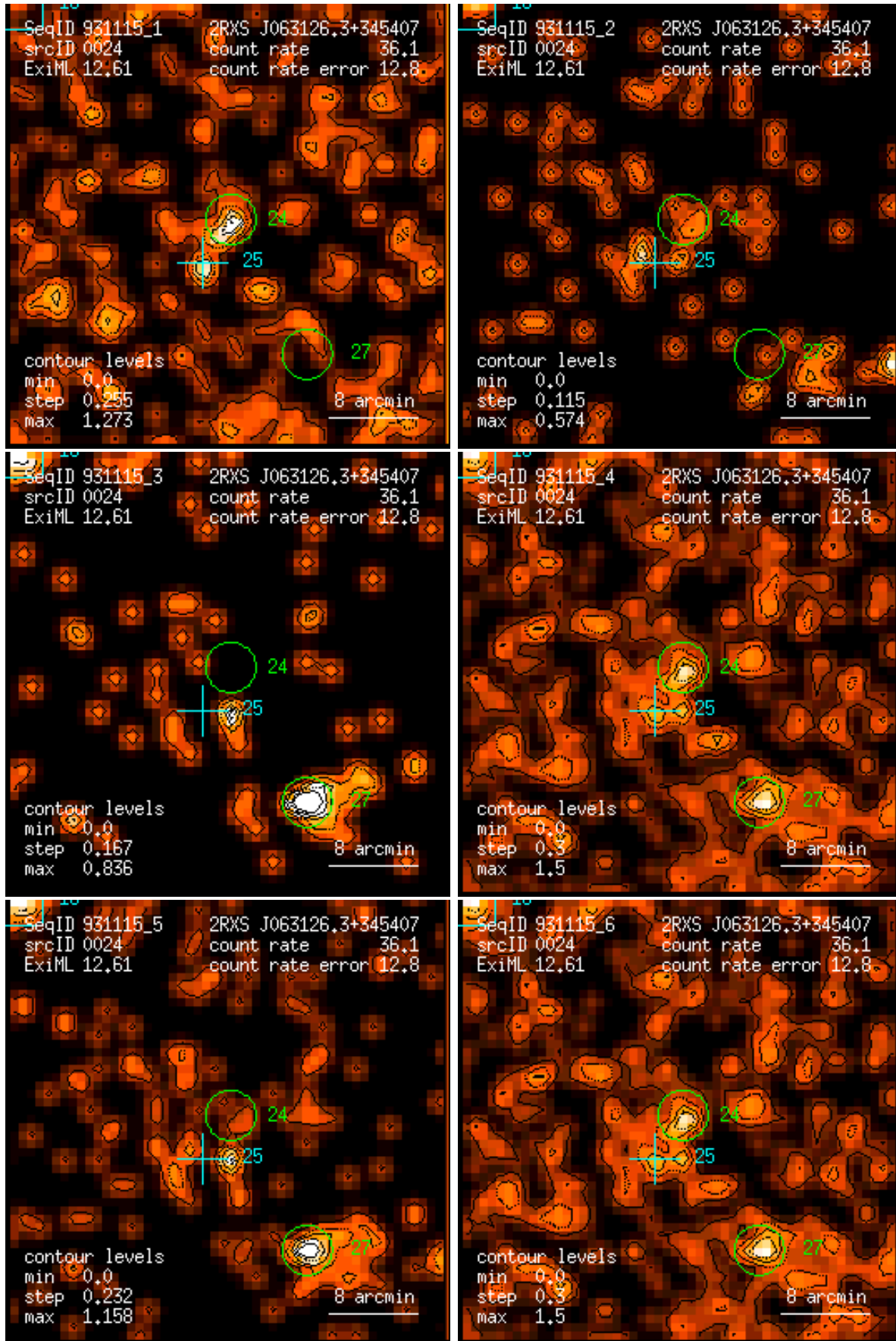
Figure 24: RASS 931115: detection 0024: band rate images, Gaussian filter: (1) PSPC channels 11 – 41, (2) 52 – 90, (3) 91 – 201, (4) 11 – 235, (5) 52 – 201, (6) 11 – 201. Broad band rates in counts/ks. Band rate contour levels in counts/ks/arcmin 2 .
