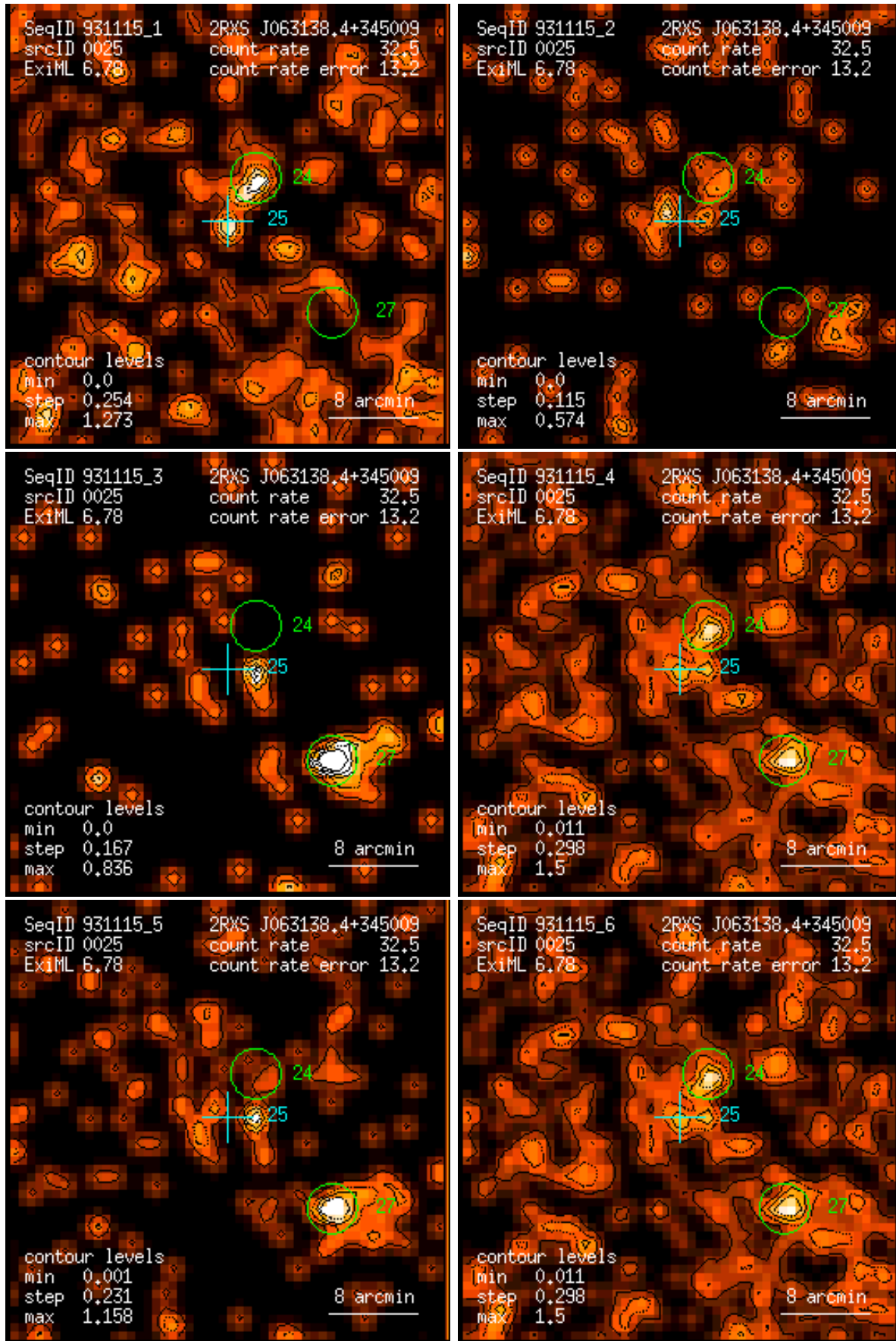
Figure 25: RASS 931115: detection 0025: band rate images, Gaussian filter: (1) PSPC channels 11 – 41, (2) 52 – 90, (3) 91 – 201, (4) 11 – 235, (5) 52 – 201, (6) 11 – 201. Broad band rates in counts/ks. Band rate contour levels in counts/ks/arcmin 2 .
