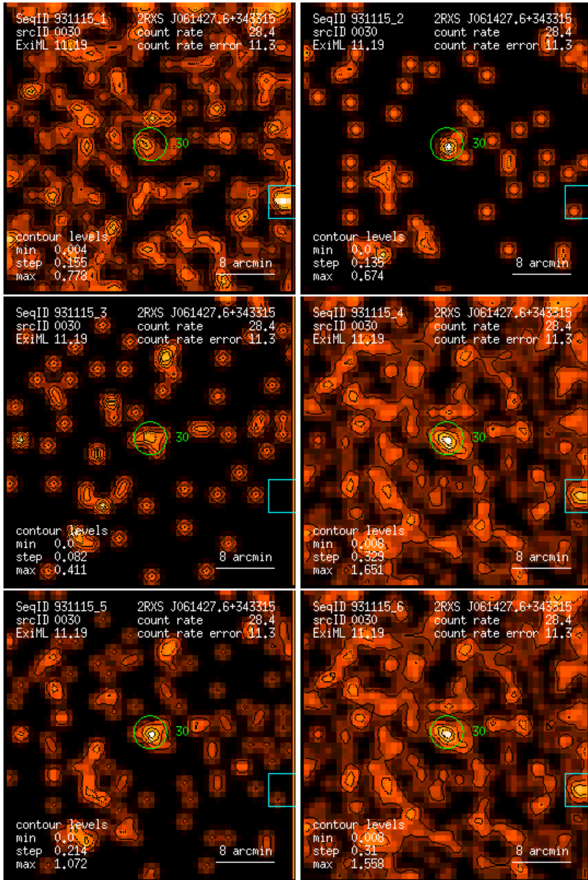
Figure 30: RASS 931115: detection 0030: band rate images, Gaussian filter: (1) PSPC channels 11 – 41, (2) 52 – 90, (3) 91 – 201, (4) 11 – 235, (5) 52 – 201, (6) 11 – 201. Broad band rates in counts/ks. Band rate contour levels in counts/ks/arcmin 2 .
