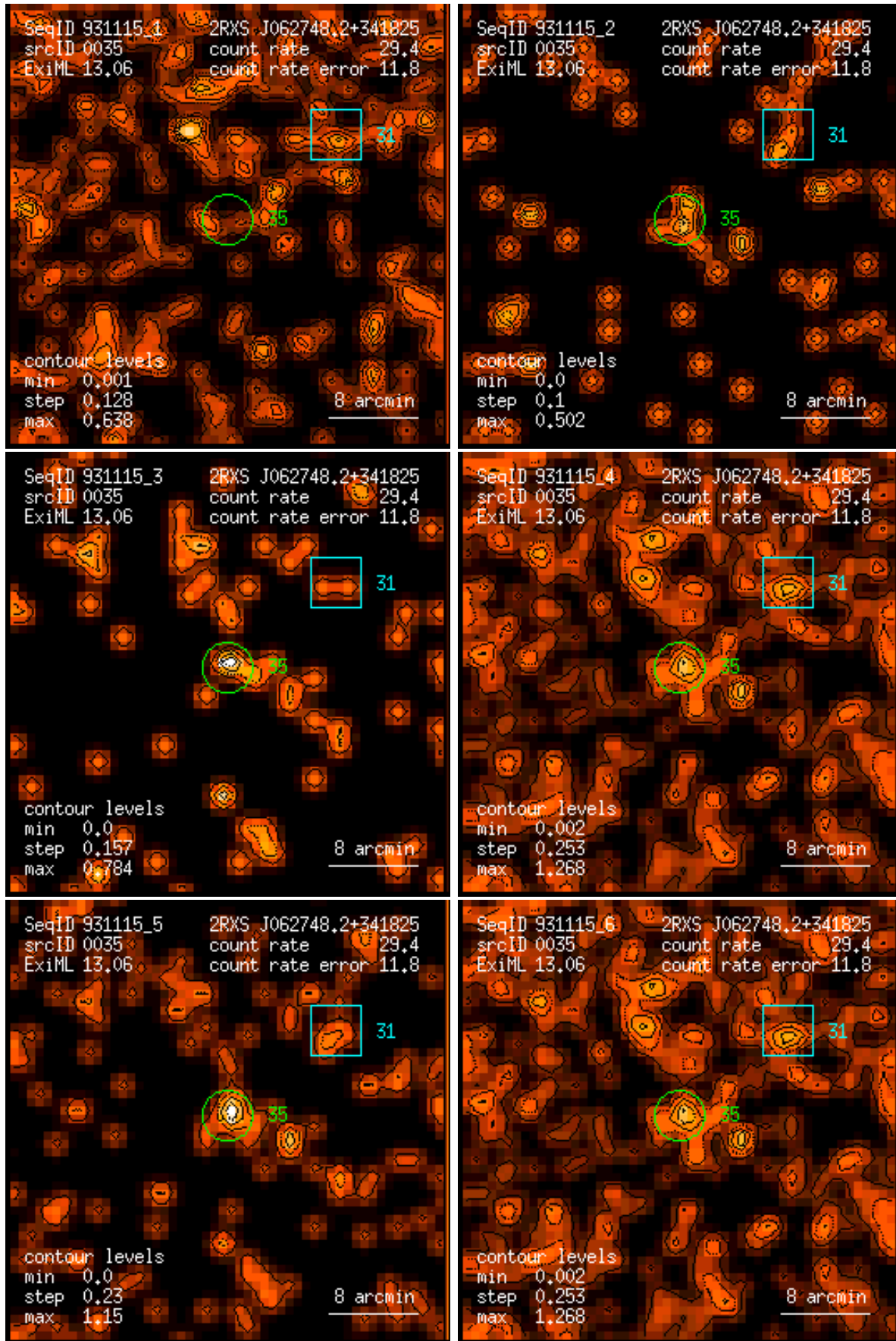
Figure 35: RASS 931115: detection 0035: band rate images, Gaussian filter: (1) PSPC channels 11 – 41, (2) 52 – 90, (3) 91 – 201, (4) 11 – 235, (5) 52 – 201, (6) 11 – 201. Broad band rates in counts/ks. Band rate contour levels in counts/ks/arcmin 2 .
