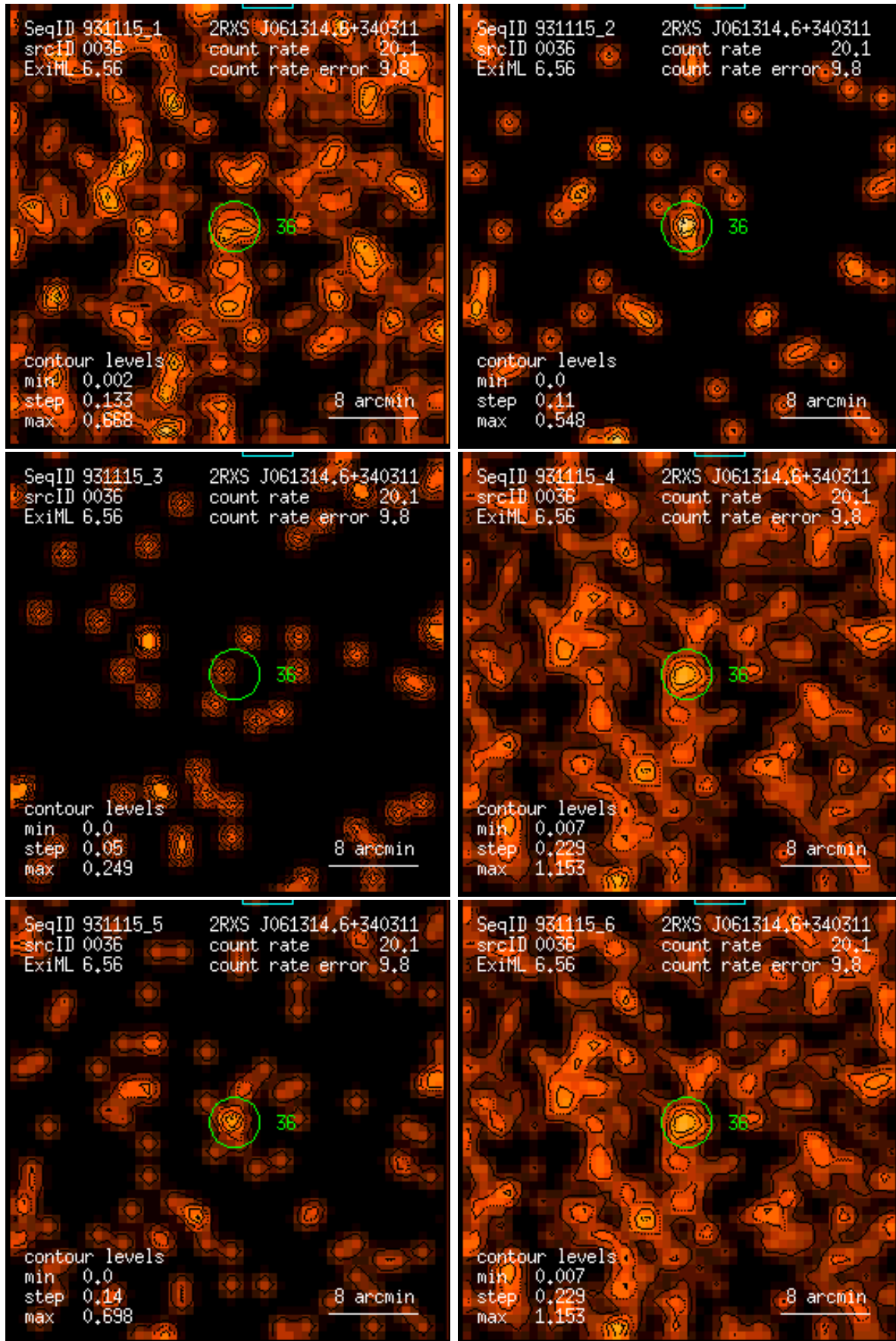
Figure 36: RASS 931115: detection 0036: band rate images, Gaussian filter: (1) PSPC channels 11 – 41, (2) 52 – 90, (3) 91 – 201, (4) 11 – 235, (5) 52 – 201, (6) 11 – 201. Broad band rates in counts/ks. Band rate contour levels in counts/ks/arcmin 2 .
