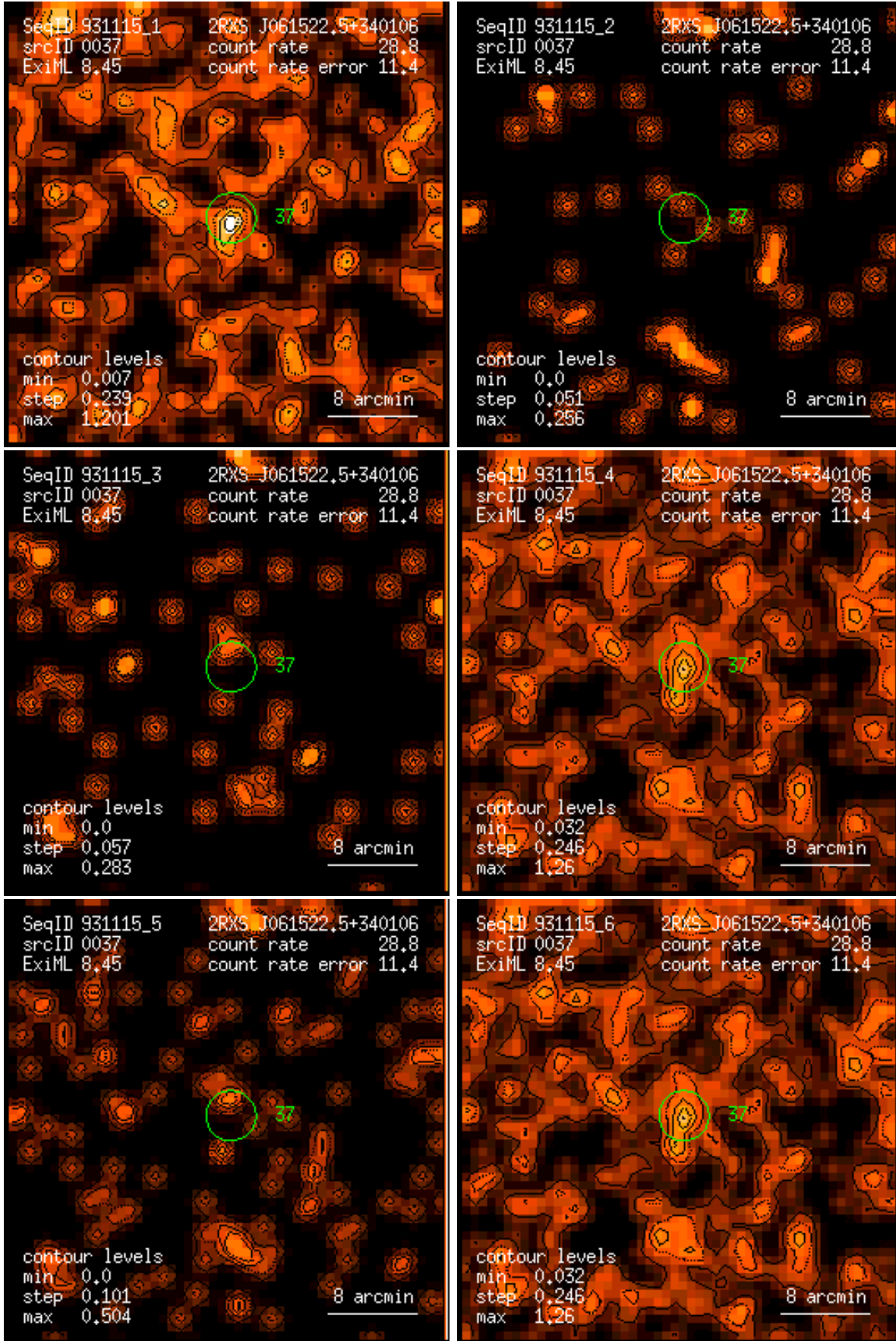
Figure 37: RASS 931115: detection 0037: band rate images, Gaussian filter: (1) PSPC channels 11 – 41, (2) 52 – 90, (3) 91 – 201, (4) 11 – 235, (5) 52 – 201, (6) 11 – 201. Broad band rates in counts/ks. Band rate contour levels in counts/ks/arcmin 2 .
