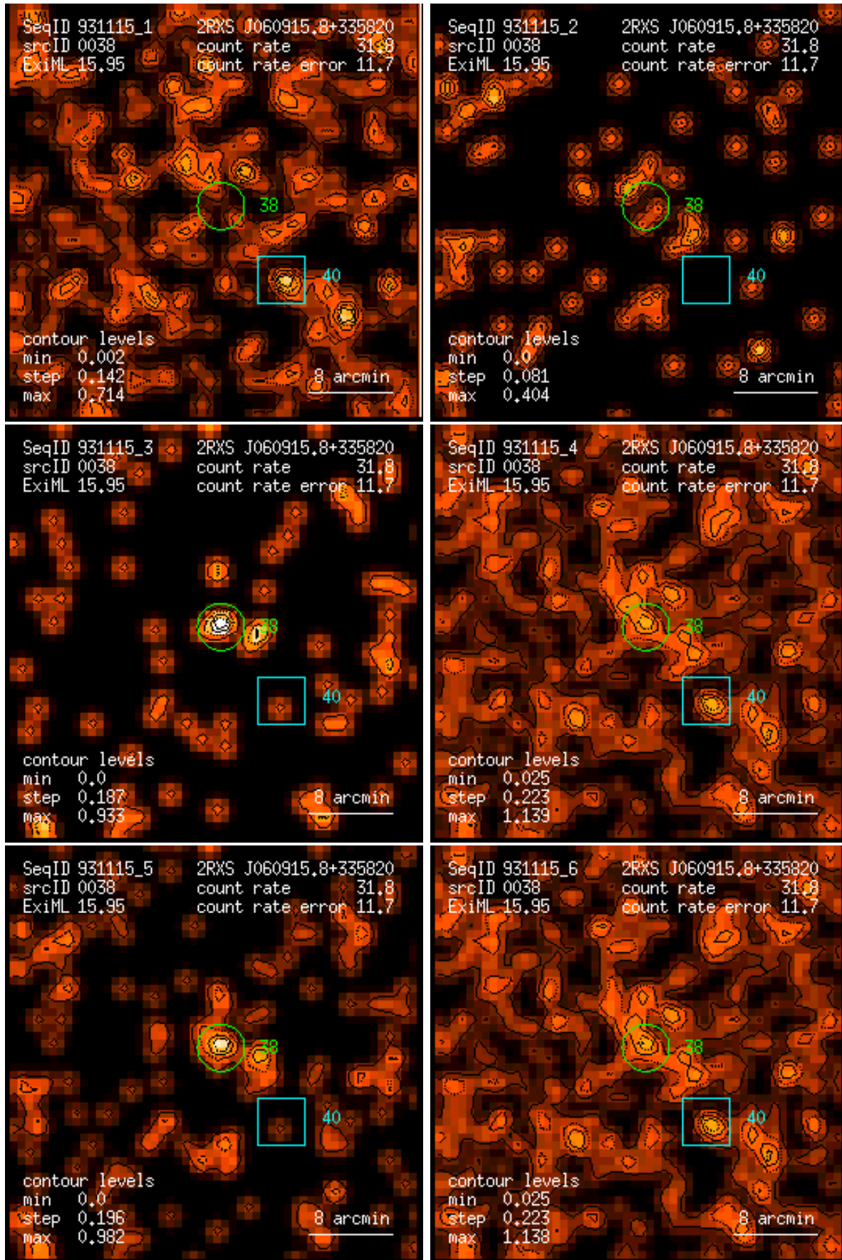
Figure 38: RASS 931115: detection 0038: band rate images, Gaussian filter: (1) PSPC channels 11 – 41, (2) 52 – 90, (3) 91 – 201, (4) 11 – 235, (5) 52 – 201, (6) 11 – 201. Broad band rates in counts/ks. Band rate contour levels in counts/ks/arcmin 2 .
