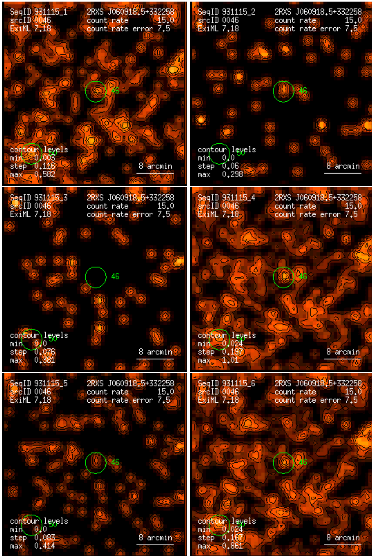
Figure 46: RASS 931115: detection 0046: band rate images, Gaussian filter: (1) PSPC channels 11 – 41, (2) 52 – 90, (3) 91 – 201, (4) 11 – 235, (5) 52 – 201, (6) 11 – 201. Broad band rates in counts/ks. Band rate contour levels in counts/ks/arcmin 2 .
