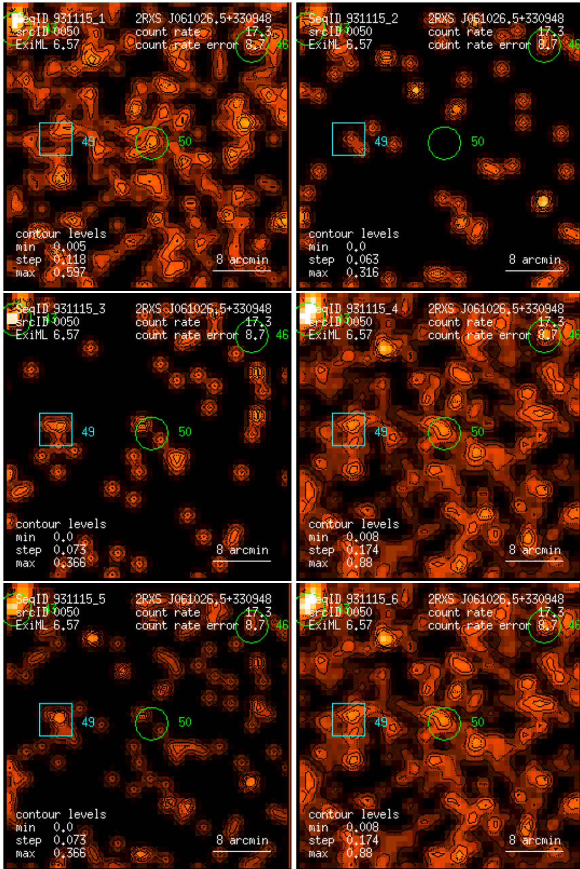
Figure 50: RASS 931115: detection 0050: band rate images, Gaussian filter: (1) PSPC channels 11 – 41, (2) 52 – 90, (3) 91 – 201, (4) 11 – 235, (5) 52 – 201, (6) 11 – 201. Broad band rates in counts/ks. Band rate contour levels in counts/ks/arcmin 2 .
