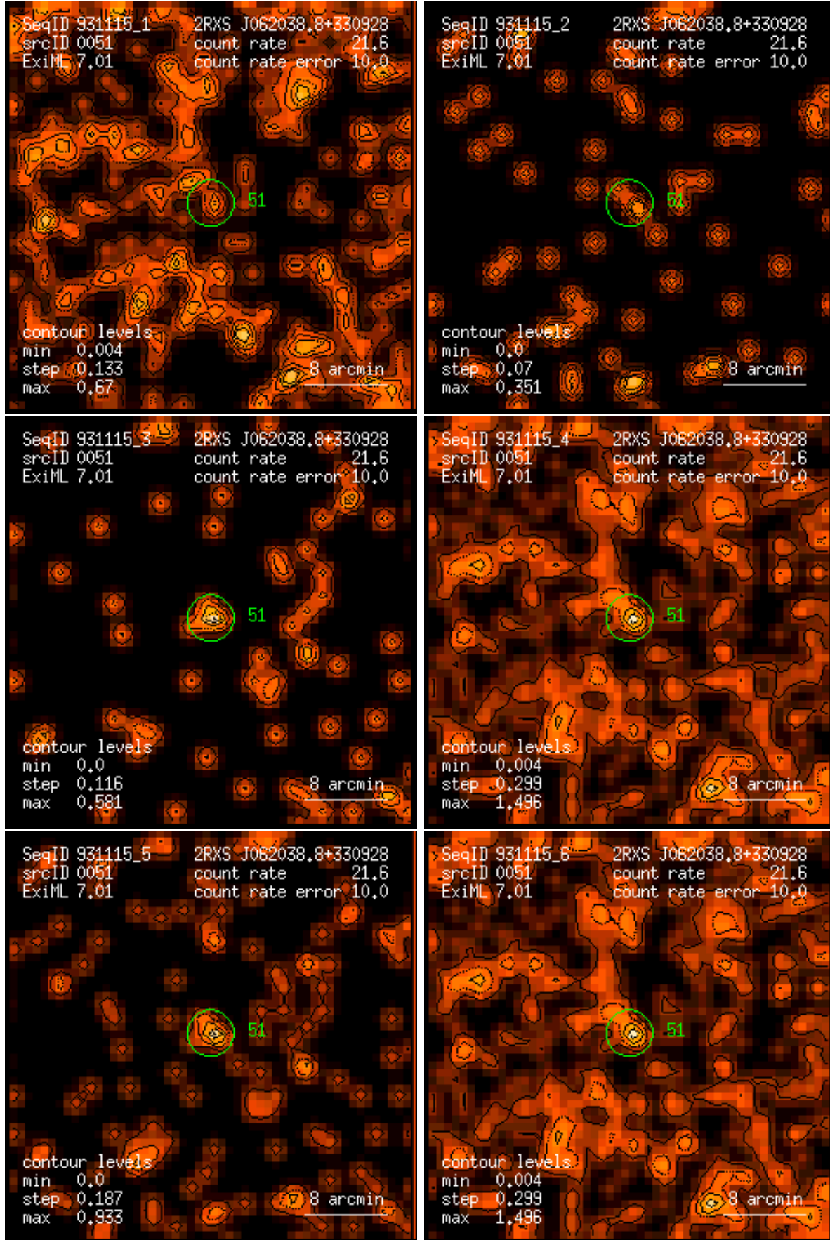
Figure 51: RASS 931115: detection 0051: band rate images, Gaussian filter: (1) PSPC channels 11 – 41, (2) 52 – 90, (3) 91 – 201, (4) 11 – 235, (5) 52 – 201, (6) 11 – 201. Broad band rates in counts/ks. Band rate contour levels in counts/ks/arcmin 2 .
