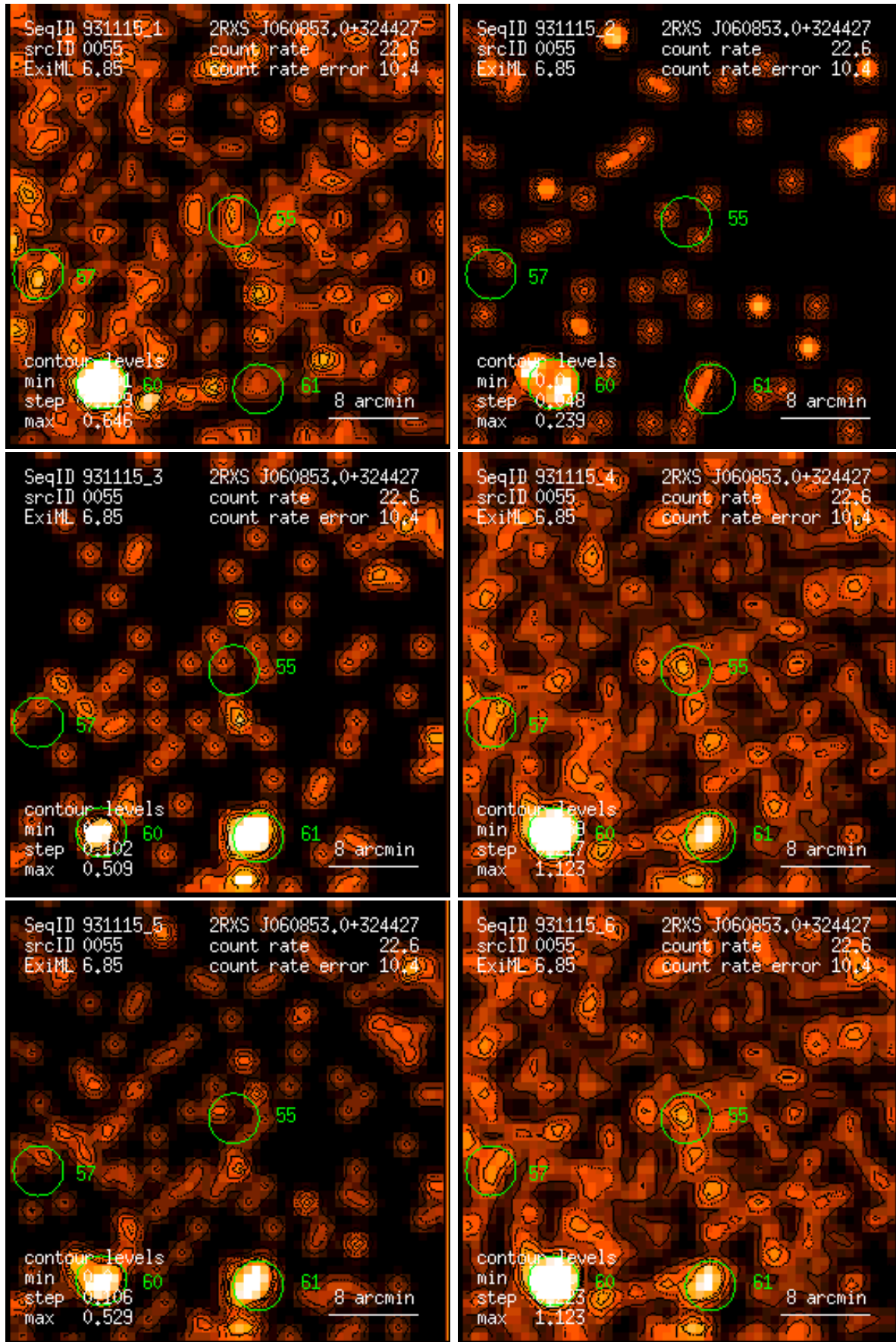
Figure 55: RASS 931115: detection 0055: band rate images, Gaussian filter: (1) PSPC channels 11 – 41, (2) 52 – 90, (3) 91 – 201, (4) 11 – 235, (5) 52 – 201, (6) 11 – 201. Broad band rates in counts/ks. Band rate contour levels in counts/ks/arcmin 2 .
